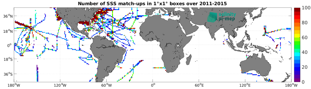
Figure 5: Number of SSS match-ups between TSG (SAMOS) SSS and the Aquarius SSS L3 OR v5 - 7-Day running - Rain mask (NASA-GSFC) SSS product for the Mid-Low Latitudes 45N-45S Pi-MEP region over 1^{\circ} \times 1^{\circ} boxes and for the full satellite product period.
