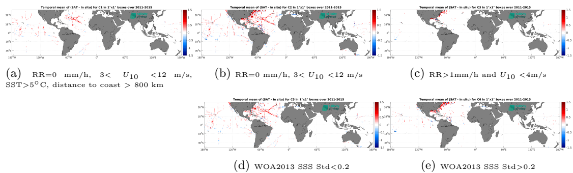
Figure 14: Temporal mean gridded over spatial boxes of size 1^\circ \times 1^\circ of \Delta SSS (Aquarius SSS L3 OR v5 - 7-Day running - Rain mask (NASA-GSFC) - TSG (SAMOS)) for 5 different subdatasets corresponding to:RR=0 mm/h, 3 < U_{10} < 12 m/s, SST >5^\circ\text{C} , distance to coast > 800 km (a), RR=0 mm/h, 3 < U_{10} < 12 m/s (b), RR >1 mm/h and U_{10} < 4 m/s (c), WOA2013 SSS Std <0.2 (d), WOA2013 SSS Std >0.2 (e).
