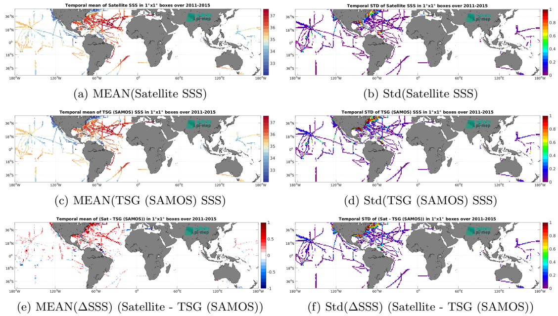
Figure 7: Temporal mean (left) and Std (right) of SSS from Aquarius SSS L3 OR v5 - 7-Day running - Rain mask (NASA-GSFC) (top), TSG (SAMOS) (middle), and of \Delta SSS (Satellite - TSG (SAMOS)). Only match-up pairs are used to generate these maps.
