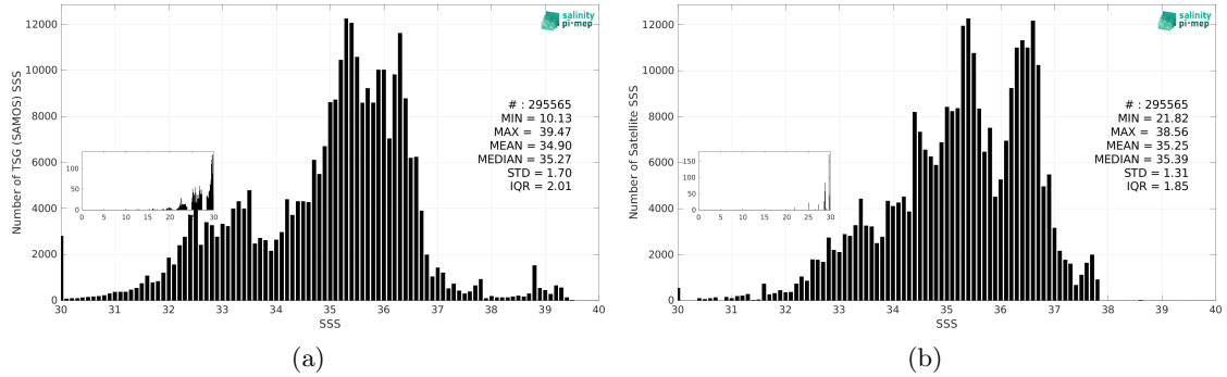
Figure 3: Histograms of SSS from TSG (SAMOS) (a) and Aquarius SSS L3 OR v5 - 7-Day running - Rain mask (NASA-GSFC) (b) considering all match-up pairs per bins of 0.1 over the Mid-Low Latitudes 45N-45S Pi-MEP region and for the full satellite product period.
