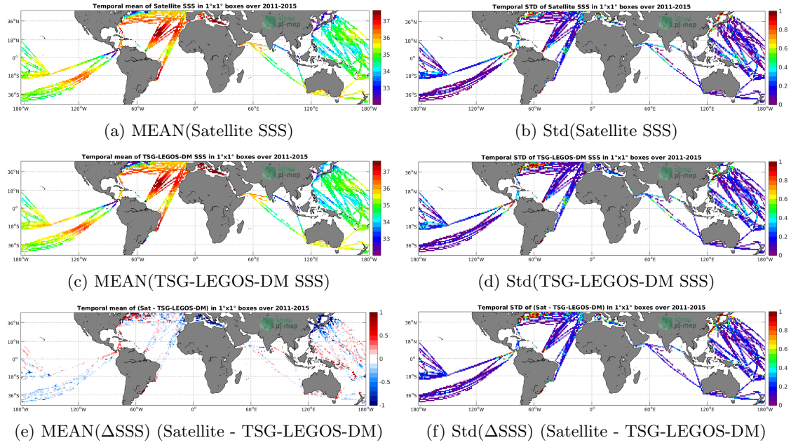
Figure 6: Temporal mean (left) and Std (right) of SSS from Aquarius-L3-OR-V5-7DAY-RUNNING-RAIN-MASK-1DEG (top), TSG-LEGOS-DM (middle), and of \Delta SSS (Satellite - TSG-LEGOS-DM). Only match-up pairs are used to generate these maps.
