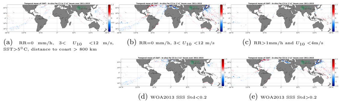
Figure 12: Temporal mean gridded over spatial boxes of size 1^\circ \times 1^\circ of \Delta SSS (Aquarius-L3-OR-V5-7DAY-RUNNING-RAIN-MASK-1DEG - TSG-LEGOS-DM) for 5 different subdatasets corresponding to: RR=0 mm/h, 3 < U_{10} < 12 m/s, SST > 5^\circ\text{C} , distance to coast > 800 km (a), RR=0 mm/h, 3 < U_{10} < 12 m/s (b), RR > 1 mm/h and U_{10} < 4 m/s (c), WOA2013 SSS Std < 0.2 (d), WOA2013 SSS Std > 0.2 (e).
