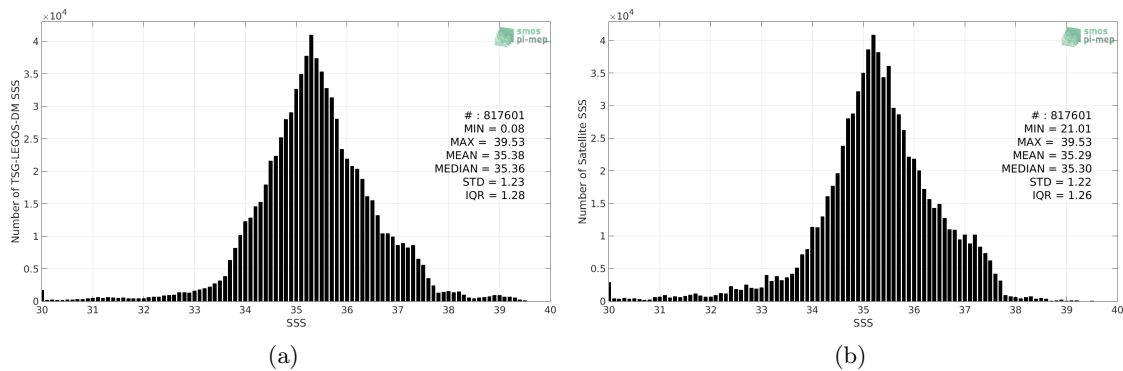
Figure 2: Histograms of SSS from TSG-LEGOS-DM (a) and Aquarius-L3-OR-V5-7DAY-RUNNING-RAIN-MASK-1DEG (b) considering all match-up pairs per bins of 0.1 over the Mid-Low Latitudes 45N-45S Pi-MEP region and for the full satellite product period.
