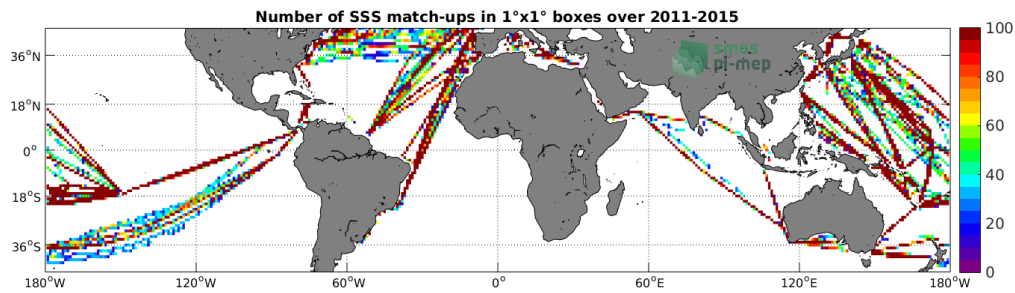
Figure 4: Number of SSS match-ups between TSG-LEGOS-DM SSS and the Aquarius-L3-OR-V5-7DAY-RUNNING-RAIN-MASK-1DEG SSS product for the Mid-Low Latitudes 45N-45S Pi-MEP region over 1^\circ \times 1^\circ boxes and for the full satellite product period.
