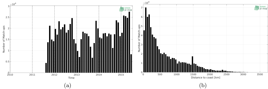
Figure 1: Number of match-ups between TSG-LEGOS-DM and Aquarius-L3-OR-V5-7DAY-RUNNING-RAIN-MASK-1DEG SSS as a function of time (a) and as function of the distance to coast (b) over the Mid-Low Latitudes 45N-45S Pi-MEP region and for the full satellite product period.
