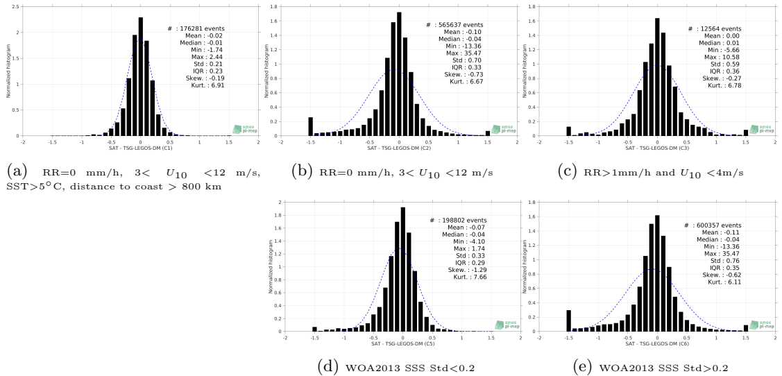
Figure 13: Normalized histogram of \Delta SSS (Aquarius-L3-OR-V5-7DAY-RUNNING-RAIN-MASK-1DEG - TSG-LEGOS-DM) for 5 different subdatasets corresponding to: RR=0 mm/h, 3 < U_{10} < 12 m/s, SST >5^\circ\text{C} , distance to coast > 800 km (a), RR=0 mm/h, 3 < U_{10} < 12 m/s (b), RR >1 mm/h and U_{10} < 4 m/s (c), WOA2013 SSS Std <0.2 (d), WOA2013 SSS Std >0.2 (e).
