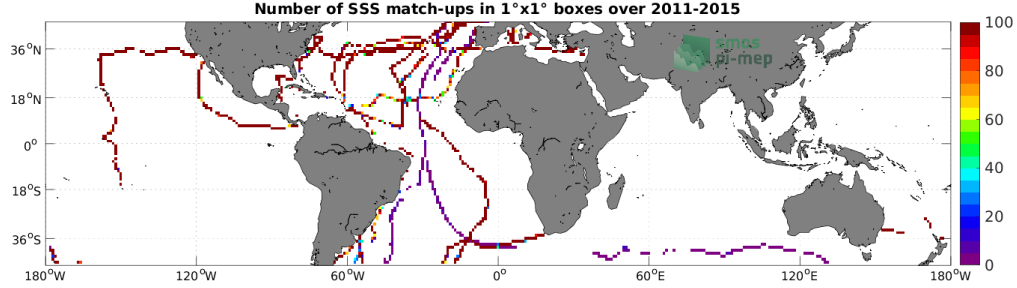
Figure 4: Number of SSS match-ups between TSG (GOSUD-Sailing-ship) SSS and the Aquarius SSS L3 OR v5 - 7-Day running - Rain mask (NASA-GSFC) SSS product for the Mid-Low Latitudes 45N-45S Pi-MEP region over 1^\circ \times 1^\circ boxes and for the full satellite product period.
