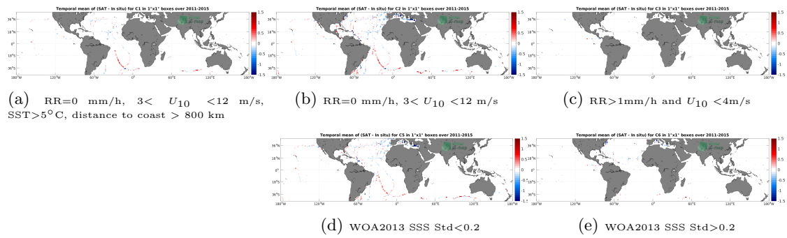
Figure 12: Temporal mean gridded over spatial boxes of size 1^\circ \times 1^\circ of \Delta SSS (Aquarius SSS L3 OR v5 - 7-Day running - Rain mask (NASA-GSFC) - TSG (GOSUD-Sailing-ship)) for 5 different subdatasets corresponding to:RR=0 mm/h, 3 < U_{10} < 12 m/s, SST >5^\circ C, distance to coast > 800 km (a), RR=0 mm/h, 3 < U_{10} < 12 m/s (b), RR >1 mm/h and U_{10} < 4 m/s (c), WOA2013 SSS Std <0.2 (d), WOA2013 SSS Std >0.2 (e).
