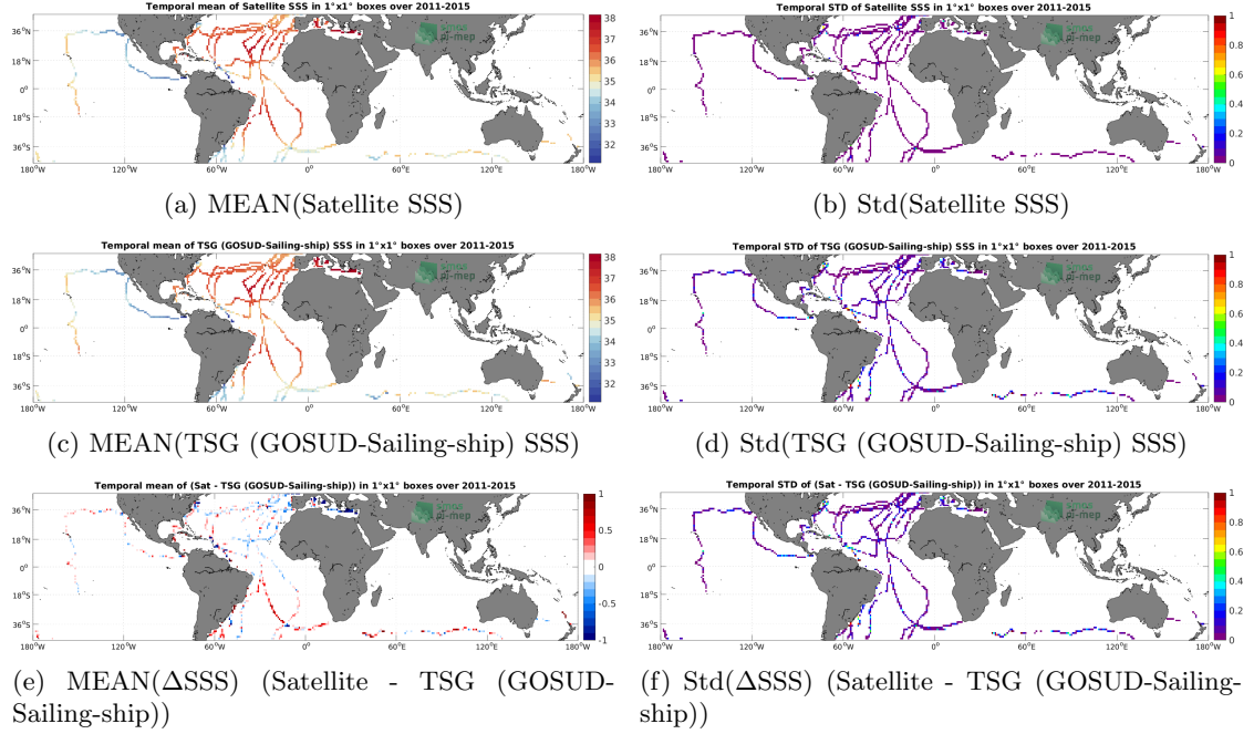
Figure 6: Temporal mean (left) and Std (right) of SSS from Aquarius SSS L3 OR v5 - 7-Day running - Rain mask (NASA-GSFC) (top), TSG (GOSUD-Sailing-ship) (middle), and of \Delta SSS (Satellite - TSG (GOSUD-Sailing-ship)). Only match-up pairs are used to generate these maps.
