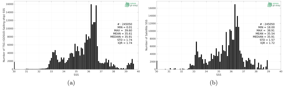
Figure 2: Histograms of SSS from TSG (GOSUD-Sailing-ship) (a) and Aquarius SSS L3 OR v5 - 7-Day running - Rain mask (NASA-GSFC) (b) considering all match-up pairs per bins of 0.1 over the Mid-Low Latitudes 45N-45S Pi-MEP region and for the full satellite product period.
