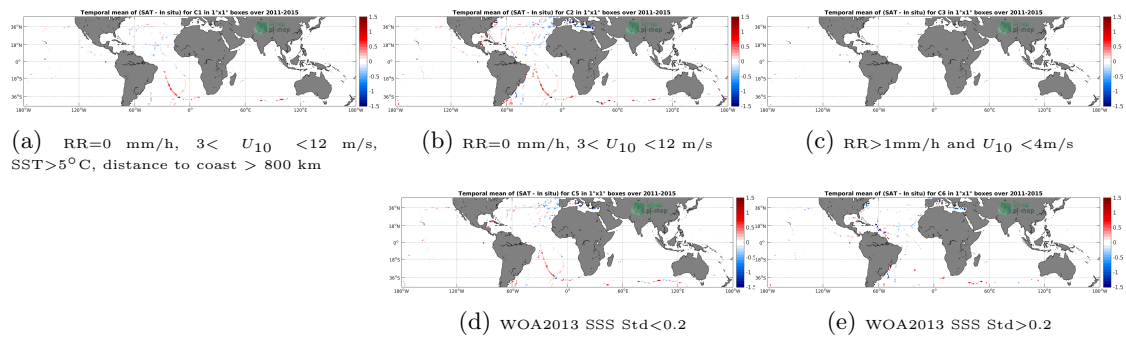
Figure 12: Temporal mean gridded over spatial boxes of size 1^\circ \times 1^\circ of \Delta\text{SSS} (Aquarius SSS L3 OR v5 - 7-Day running - Rain mask (NASA-GSFC) - TSG (GOSUD-Sailing-ship)) for 5 different subdatasets corresponding to: RR=0 mm/h, 3 < U_{10} < 12 m/s, SST > 5°C, distance to coast > 800 km (a), RR=0 mm/h, 3 < U_{10} < 12 m/s (b), RR > 1mm/h and U_{10} < 4 m/s (c), WOA2013 SSS Std < 0.2 (d), WOA2013 SSS Std > 0.2 (e).
