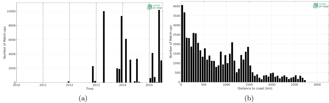
Figure 1: Number of match-ups between TSG-GOSUD-Sailing-ship and Aquarius-L3-OR-V5-7DAY-RUNNING-RAIN-MASK-1DEG SSS as a function of time (a) and as function of the distance to coast (b) over the Mid-Low Latitudes 45N-45S Pi-MEP region and for the full satellite product period.
