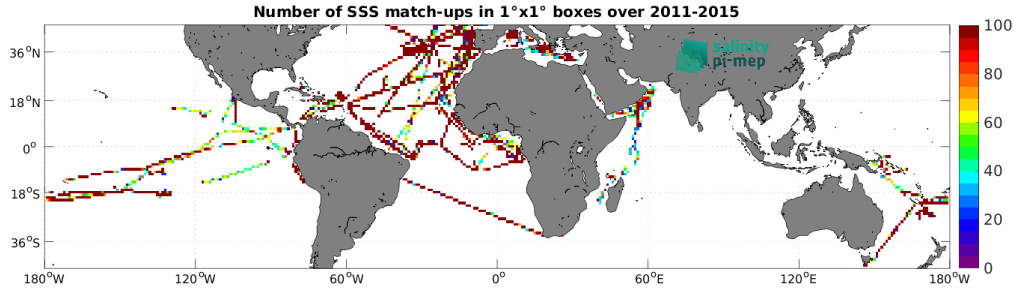
Figure 5: Number of SSS match-ups between TSG (GOSUD-Research-vessel) SSS and the Aquarius SSS L3 OR v5 - 7-Day running - Rain mask (NASA-GSFC) SSS product for the Mid-Low Latitudes 45N-45S Pi-MEP region over 1^\circ \times 1^\circ boxes and for the full satellite product period.
