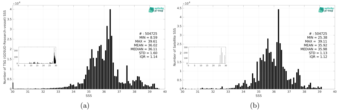
Figure 3: Histograms of SSS from TSG (GOSUD-Research-vessel) (a) and Aquarius SSS L3 OR v5 - 7-Day running - Rain mask (NASA-GSFC) (b) considering all match-up pairs per bins of 0.1 over the Mid-Low Latitudes 45N-45S Pi-MEP region and for the full satellite product period.
