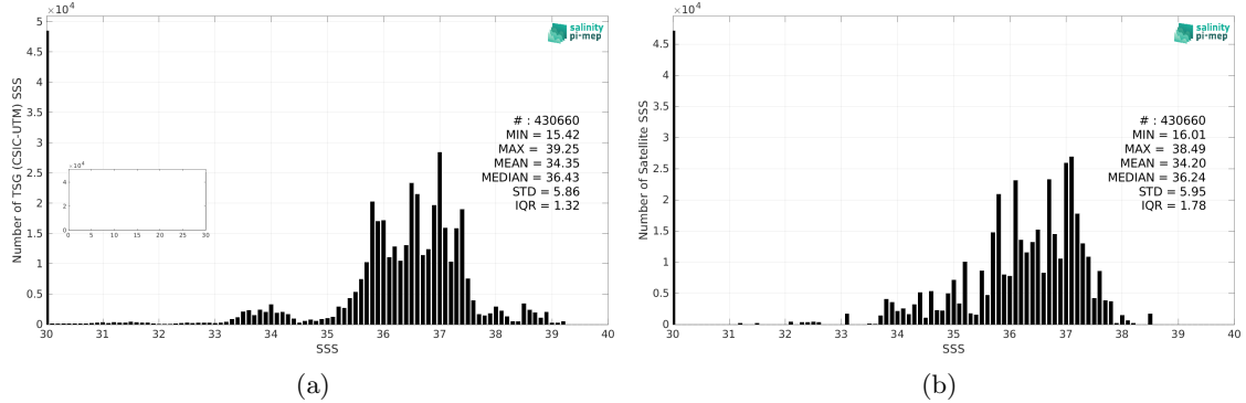
Figure 2: Histograms of SSS from TSG (CSIC-UTM) (a) and Aquarius SSS L3 OR v5 - 7-Day running - Rain mask (NASA-GSFC) (b) considering all match-up pairs per bins of 0.1 over the Mid-Low Latitudes 45N-45S Pi-MEP region and for the full satellite product period.
