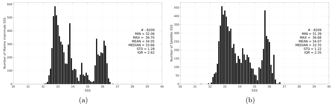
Figure 3: Histograms of SSS from Marine mammals (a) and Aquarius SSS L3 OR v5 - 7-Day running - Rain mask (NASA-GSFC) (b) considering all match-up pairs per bins of 0.1 over the Mid-Low Latitudes 45N-45S Pi-MEP region and for the full satellite product period.
