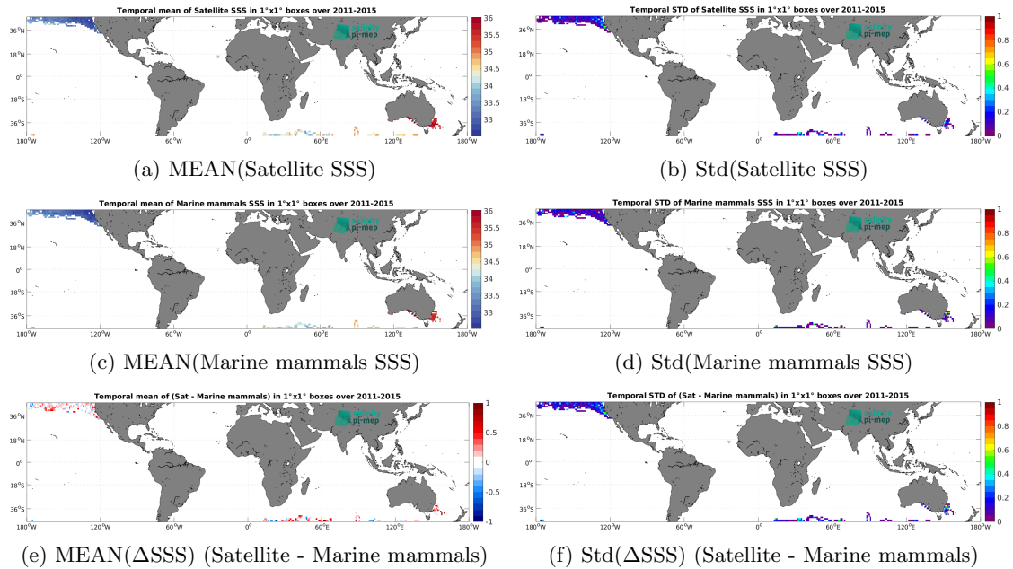
Figure 7: Temporal mean (left) and Std (right) of SSS from Aquarius SSS L3 OR v5 - 7-Day running - Rain mask (NASA-GSFC) (top), Marine mammals (middle), and of \Delta SSS (Satellite - Marine mammals). Only match-up pairs are used to generate these maps.
