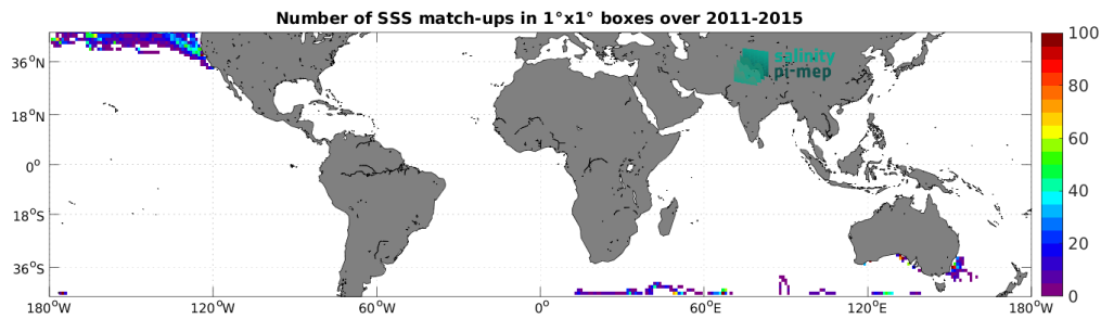
Figure 5: Number of SSS match-ups between Marine mammals SSS and the Aquarius SSS L3 OR v5 - 7-Day running - Rain mask (NASA-GSFC) SSS product for the Mid-Low Latitudes 45N-45S Pi-MEP region over 1^\circ \times 1^\circ boxes and for the full satellite product period.
