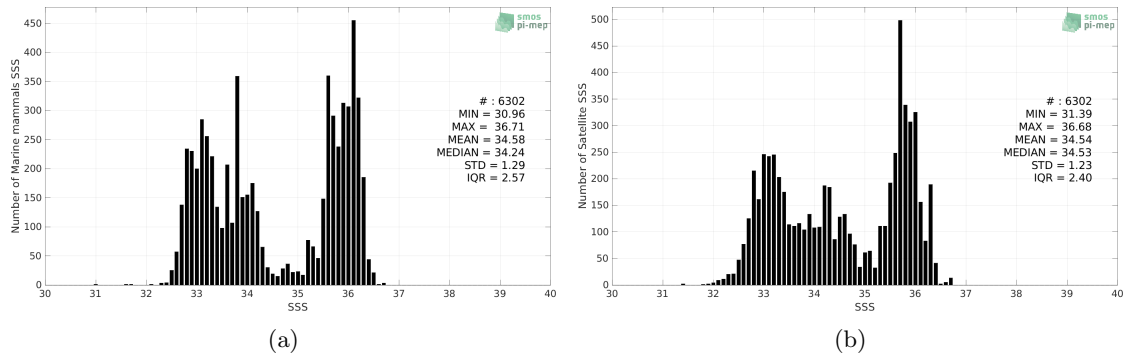
Figure 2: Histograms of SSS from Marine mammals (a) and Aquarius SSS L3 OR v5 - 7-Day running - Rain mask (NASA-GSFC) (b) considering all match-up pairs per bins of 0.1 over the Mid-Low Latitudes 45N-45S Pi-MEP region and for the full satellite product period.
