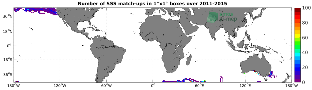
Figure 4: Number of SSS match-ups between Marine mammals SSS and the Aquarius SSS L3 OR v5 - 7-Day running - Rain mask (NASA-GSFC) SSS product for the Mid-Low Latitudes 45N-45S Pi-MEP region over 1^\circ \times 1^\circ boxes and for the full satellite product period.
