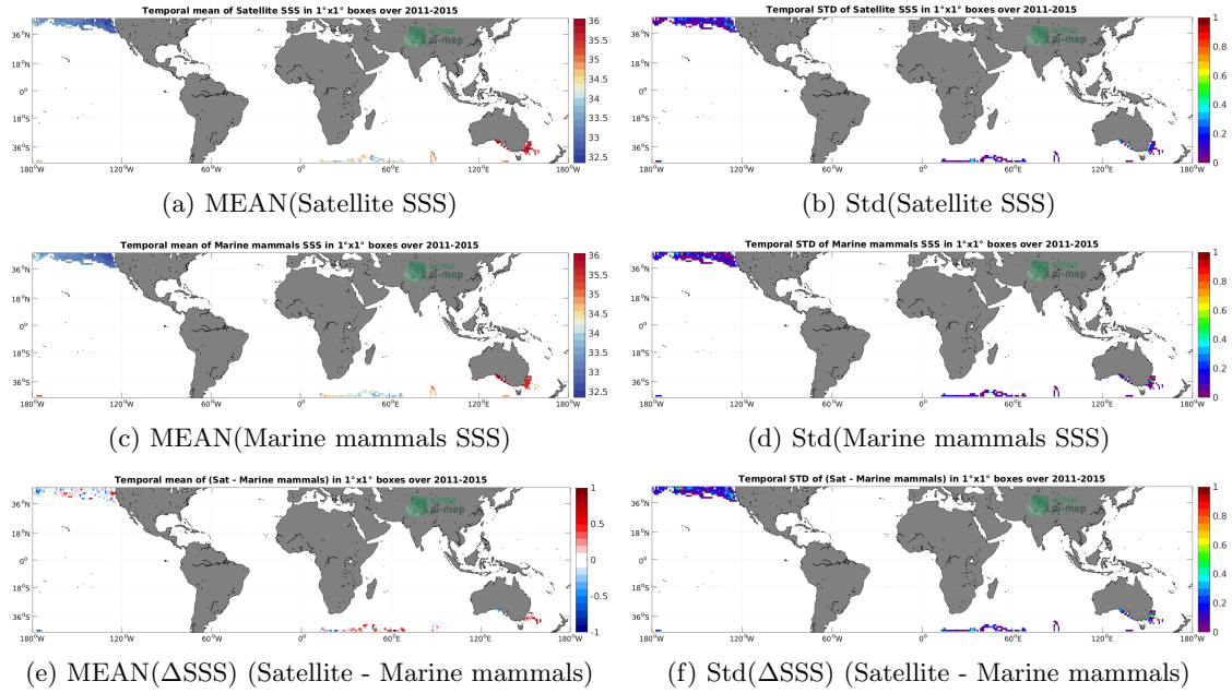
Figure 6: Temporal mean (left) and Std (right) of SSS from Aquarius SSS L3 OR v5 - 7-Day running - Rain mask (NASA-GSFC) (top), Marine mammals (middle), and of \Delta SSS (Satellite - Marine mammals). Only match-up pairs are used to generate these maps.
