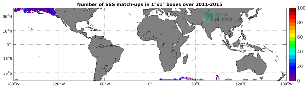
Figure 4: Number of SSS match-ups between Sea mammals SSS and the Aquarius-L3-OR-V5-7DAY-RUNNING-RAIN-MASK-1DEG SSS product for the Mid-Low Latitudes 45N-45S Pi-MEP region over 1^\circ \times 1^\circ boxes and for the full satellite product period.
