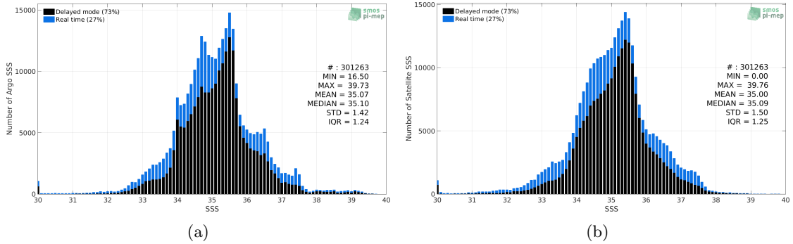
Figure 2: Histograms of SSS from Argos (a) and Aquarius-L3-OR-V5-7DAY-RUNNING-RAIN-MASK-1DEG (b) considering all match-up pairs per bins of 0.1 over the Mid-Low Latitudes 45N-45S Pi-MEP region and for the full satellite product period.
