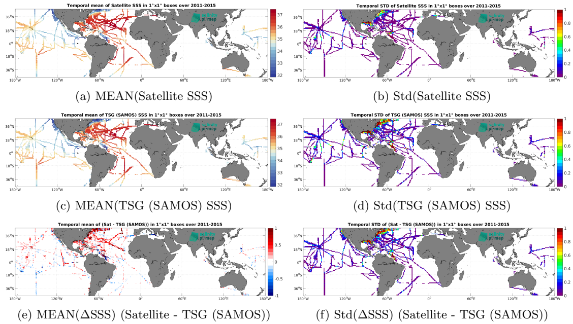
Figure 6: Temporal mean (left) and Std (right) of SSS from Aquarius SSS L3 OR v5 - Monthly (NASA-GSFC) (top), TSG (SAMOS) (middle), and of \Delta SSS (Satellite - TSG (SAMOS)). Only match-up pairs are used to generate these maps.
