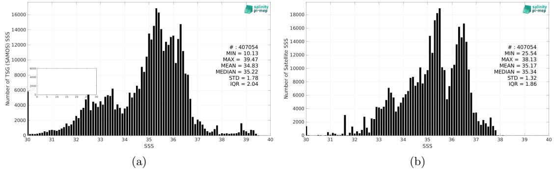
Figure 2: Histograms of SSS from TSG (SAMOS) (a) and Aquarius SSS L3 OR v5 - Monthly (NASA-GSFC) (b) considering all match-up pairs per bins of 0.1 over the Mid-Low Latitudes 45N-45S Pi-MEP region and for the full satellite product period.
