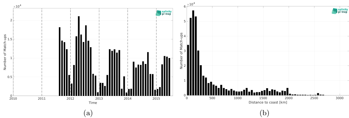
Figure 1: Number of match-ups between TSG (SAMOS) and Aquarius SSS L3 OR v5 - Monthly (NASA-GSFC) SSS as a function of time (a) and as function of the distance to coast (b) over the Mid-Low Latitudes 45N-45S Pi-MEP region and for the full satellite product period.
