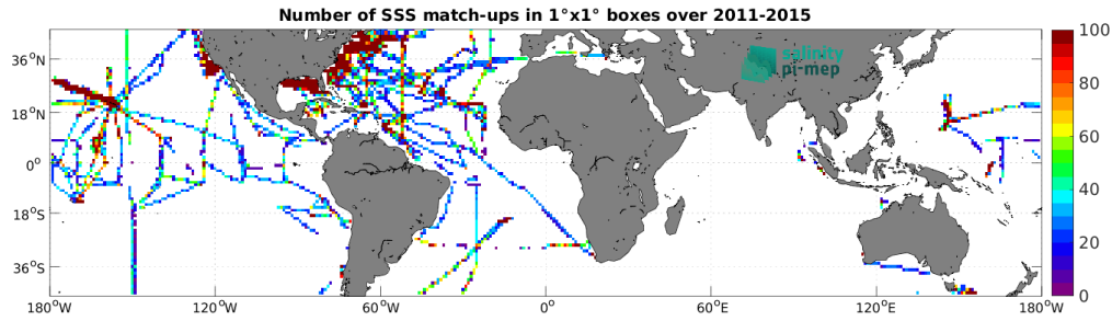
Figure 4: Number of SSS match-ups between TSG (SAMOS) SSS and the Aquarius SSS L3 OR v5 - Monthly (NASA-GSFC) SSS product for the Mid-Low Latitudes 45N-45S Pi-MEP region over 1^\circ \times 1^\circ boxes and for the full satellite product period.
