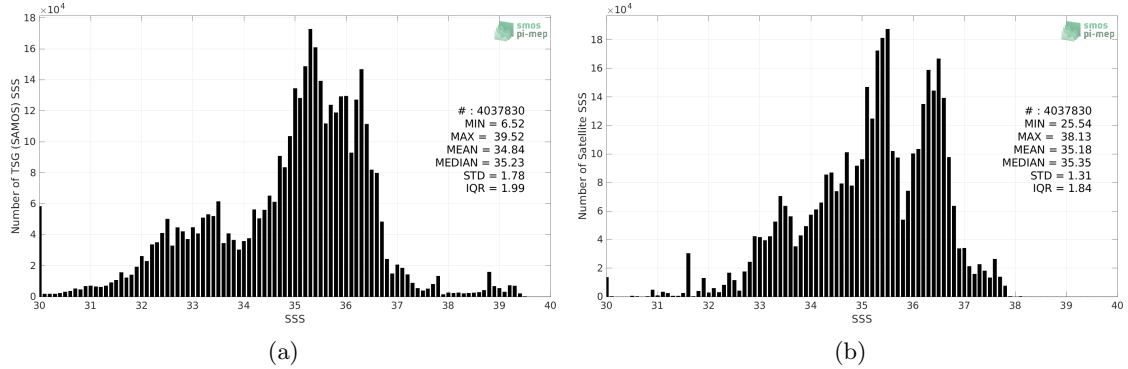
Figure 2: Histograms of SSS from TSG (SAMOS) (a) and Aquarius SSS L3 OR v5 - Monthly (NASA-GSFC) (b) considering all match-up pairs per bins of 0.1 over the Mid-Low Latitudes 45N-45S Pi-MEP region and for the full satellite product period.
