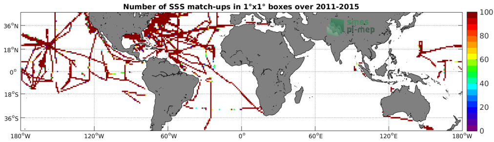
Figure 4: Number of SSS match-ups between TSG-SAMOS SSS and the Aquarius-L3-OR-V5-MONTHLY-1DEG SSS product for the Mid-Low Latitudes 45N-45S Pi-MEP region over 1^\circ \times 1^\circ boxes and for the full satellite product period.
