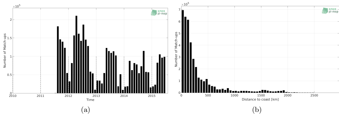
Figure 1: Number of match-ups between TSG-SAMOS and Aquarius-L3-OR-V5-MONTHLY-1DEG SSS as a function of time (a) and as function of the distance to coast (b) over the Mid-Low Latitudes 45N-45S Pi-MEP region and for the full satellite product period.
