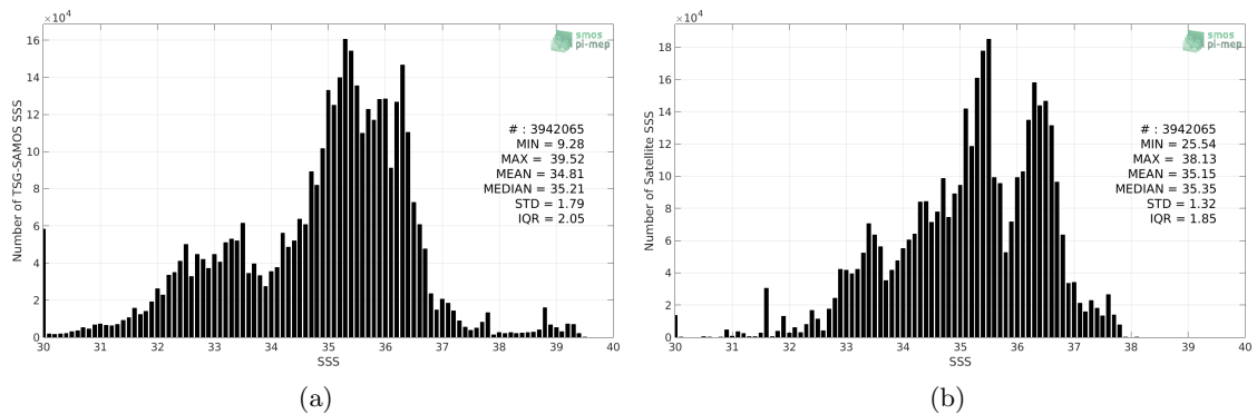
Figure 2: Histograms of SSS from TSG-SAMOS (a) and Aquarius-L3-OR-V5-MONTHLY-1DEG (b) considering all match-up pairs per bins of 0.1 over the Mid-Low Latitudes 45N-45S Pi-MEP region and for the full satellite product period.
