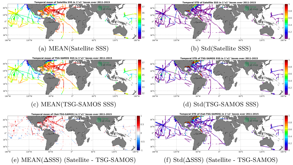
Figure 6: Temporal mean (left) and Std (right) of SSS from Aquarius-L3-OR-V5-MONTHLY-1DEG (top), TSG-SAMOS (middle), and of \Delta SSS (Satellite - TSG-SAMOS). Only match-up pairs are used to generate these maps.
