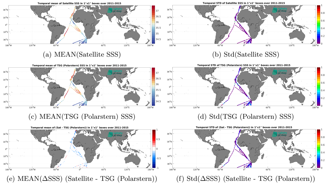
Figure 7: Temporal mean (left) and Std (right) of SSS from Aquarius SSS L3 OR v5 - Monthly (NASA-GSFC) (top), TSG (Polarstern) (middle), and of \Delta SSS (Satellite - TSG (Polarstern)). Only match-up pairs are used to generate these maps.
