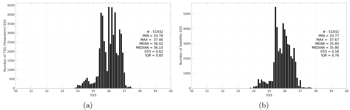
Figure 3: Histograms of SSS from TSG (Polarstern) (a) and Aquarius SSS L3 OR v5 - Monthly (NASA-GSFC) (b) considering all match-up pairs per bins of 0.1 over the Mid-Low Latitudes 45N-45S Pi-MEP region and for the full satellite product period.
