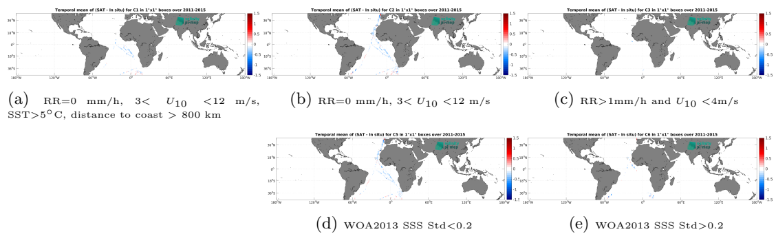
Figure 14: Temporal mean gridded over spatial boxes of size 1^\circ \times 1^\circ of \Delta\text{SSS} (Aquarius SSS L3 OR v5 - Monthly (NASA-GSFC) - TSG (Polarstern)) for 5 different subdatasets corresponding to: RR=0 mm/h, 3 < U_{10} < 12 m/s, SST > 5°C, distance to coast > 800 km (a), RR=0 mm/h, 3 < U_{10} < 12 m/s (b), RR > 1mm/h and U_{10} < 4 m/s (c), WOA2013 SSS Std < 0.2 (d), WOA2013 SSS Std > 0.2 (e).
