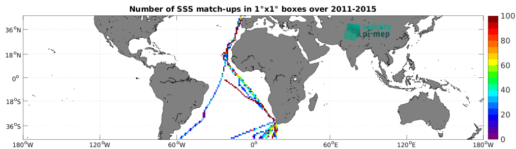
Figure 5: Number of SSS match-ups between TSG (Polarstern) SSS and the Aquarius SSS L3 OR v5 - Monthly (NASA-GSFC) SSS product for the Mid-Low Latitudes 45N-45S Pi-MEP region over 1^\circ \times 1^\circ boxes and for the full satellite product period.
