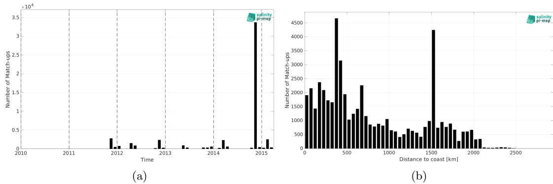
Figure 2: Number of match-ups between TSG (Polarstern) and Aquarius SSS L3 OR v5 - Monthly (NASA-GSFC) SSS as a function of time (a) and as function of the distance to coast (b) over the Mid-Low Latitudes 45N-45S Pi-MEP region and for the full satellite product period.
