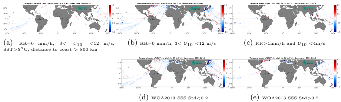
Figure 12: Temporal mean gridded over spatial boxes of size 1^\circ \times 1^\circ of \Delta\text{SSS} (Aquarius SSS L3 OR v5 - Monthly (NASA-GSFC) - TSG (LEGOS-DM)) for 5 different subdatasets corresponding to:RR=0 mm/h, 3 < U_{10} < 12 m/s, SST >5^\circ\text{C} , distance to coast > 800 km (a), RR=0 mm/h, 3 < U_{10} < 12 m/s (b), RR >1 mm/h and U_{10} < 4 m/s (c), WOA2013 SSS Std <0.2 (d), WOA2013 SSS Std >0.2 (e).
