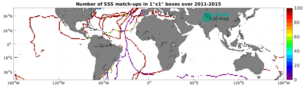
Figure 5: Number of SSS match-ups between TSG (GOSUD-Sailing-ship) SSS and the Aquarius SSS L3 OR v5 - Monthly (NASA-GSFC) SSS product for the Mid-Low Latitudes 45N-45S Pi-MEP region over 1^\circ \times 1^\circ boxes and for the full satellite product period.
