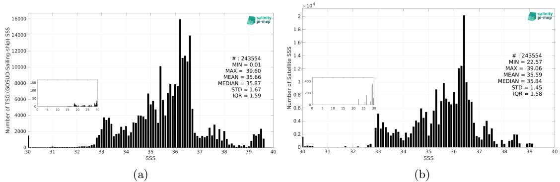
Figure 3: Histograms of SSS from TSG (GOSUD-Sailing-ship) (a) and Aquarius SSS L3 OR v5 - Monthly (NASA-GSFC) (b) considering all match-up pairs per bins of 0.1 over the Mid-Low Latitudes 45N-45S Pi-MEP region and for the full satellite product period.
