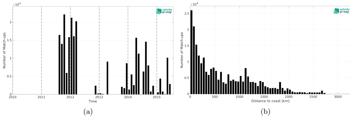
Figure 2: Number of match-ups between TSG (GOSUD-Sailing-ship) and Aquarius SSS L3 OR v5 - Monthly (NASA-GSFC) SSS as a function of time (a) and as function of the distance to coast (b) over the Mid-Low Latitudes 45N-45S Pi-MEP region and for the full satellite product period.
