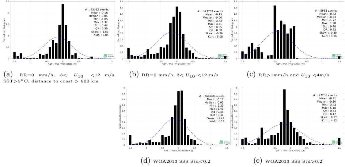
Figure 13: Normalized histogram of \Delta SSS (Aquarius SSS L3 OR v5 - Monthly (NASA-GSFC) - TSG (CSIC-UTM)) for 5 different subdatasets corresponding to: RR=0 mm/h, 3 < U_{10} < 12 m/s, SST>5°C, distance to coast > 800 km (a), RR=0 mm/h, 3 < U_{10} < 12 m/s (b), RR>1mm/h and U_{10} < 4 m/s (c), WOA2013 SSS Std<0.2 (d), WOA2013 SSS Std>0.2 (e).
