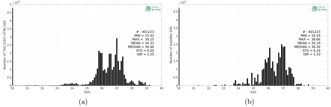
Figure 2: Histograms of SSS from TSG (CSIC-UTM) (a) and Aquarius SSS L3 OR v5 - Monthly (NASA-GSFC) (b) considering all match-up pairs per bins of 0.1 over the Mid-Low Latitudes 45N-45S Pi-MEP region and for the full satellite product period.
