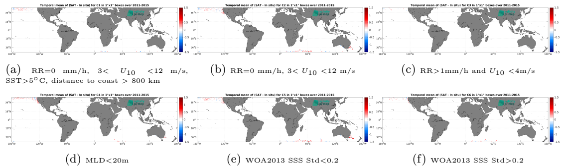
Figure 14: Temporal mean gridded over spatial boxes of size 1^\circ \times 1^\circ of \Delta SSS (Aquarius SSS L3 OR v5 - Monthly (NASA-GSFC) - Marine mammals) for 6 different subdatasets corresponding to:RR=0 mm/h, 3 < U_{10} < 12 m/s, SST>5°C, distance to coast > 800 km (a), RR=0 mm/h, 3 < U_{10} < 12 m/s (b), RR>1mm/h and U_{10} < 4 m/s (c),MLD<20m (d),WOA2013 SSS Std<0.2 (e),WOA2013 SSS Std>0.2 (f).
