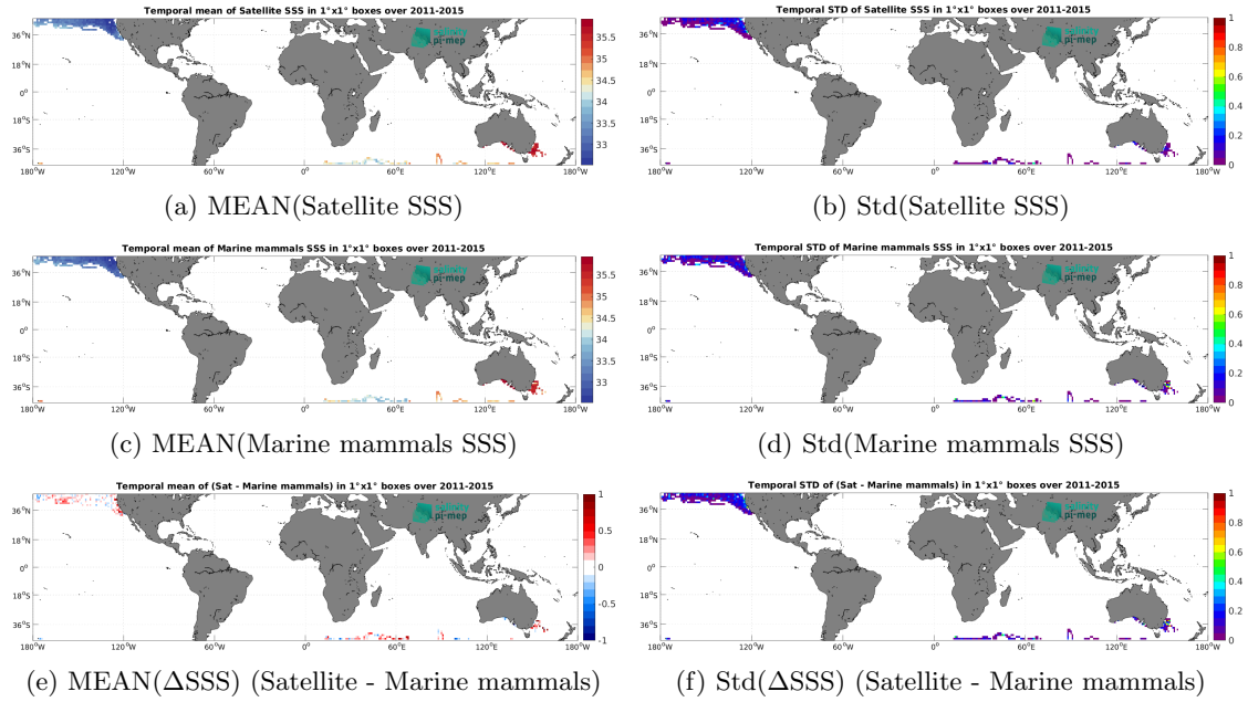
Figure 7: Temporal mean (left) and Std (right) of SSS from Aquarius SSS L3 OR v5 - Monthly (NASA-GSFC) (top), Marine mammals (middle), and of \Delta SSS (Satellite - Marine mammals). Only match-up pairs are used to generate these maps.
