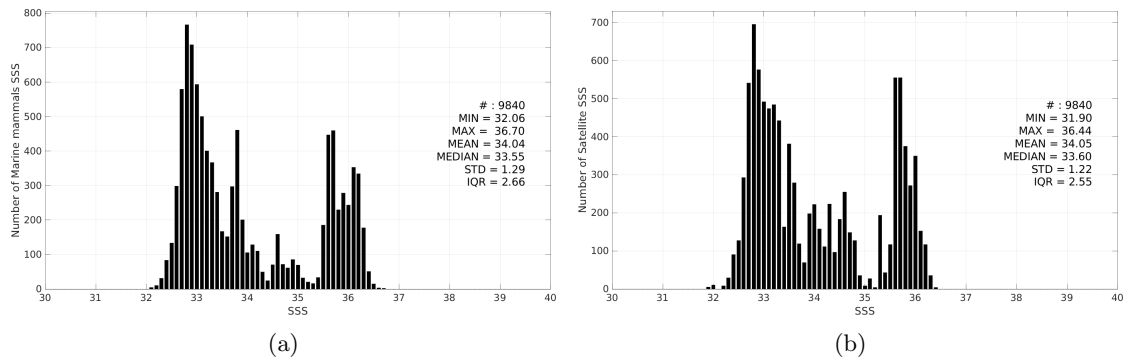
Figure 3: Histograms of SSS from Marine mammals (a) and Aquarius SSS L3 OR v5 - Monthly (NASA-GSFC) (b) considering all match-up pairs per bins of 0.1 over the Mid-Low Latitudes 45N-45S Pi-MEP region and for the full satellite product period.
