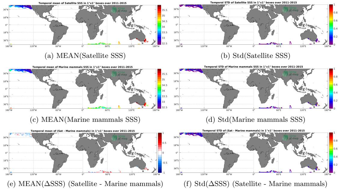
Figure 6: Temporal mean (left) and Std (right) of SSS from Aquarius SSS L3 OR v5 - Monthly (NASA-GSFC) (top), Marine mammals (middle), and of \Delta SSS (Satellite - Marine mammals). Only match-up pairs are used to generate these maps.
