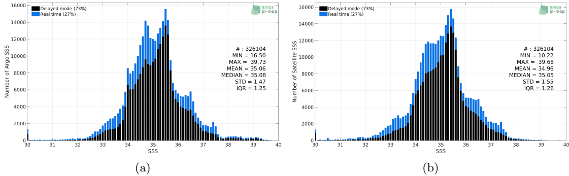
Figure 2: Histograms of SSS from Argo (a) and Aquarius-L3-OR-V5-MONTHLY-1DEG (b) considering all match-up pairs per bins of 0.1 over the Mid-Low Latitudes 45N-45S Pi-MEP region and for the full satellite product period.
