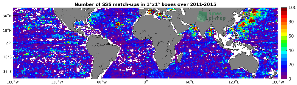
Figure 4: Number of SSS match-ups between Argo SSS and the Aquarius-L3-OR-V5-MONTHLY-1DEG SSS product for the Mid-Low Latitudes 45N-45S Pi-MEP region over 1°x1° boxes and for the full satellite product period.
