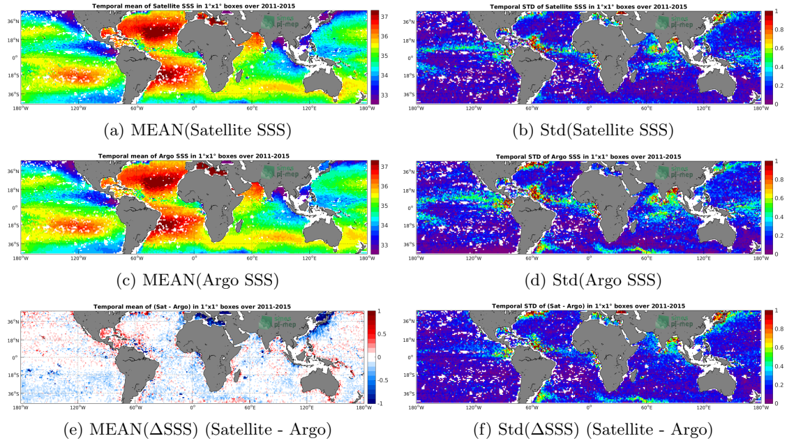
Figure 6: Temporal mean (left) and Std (right) of SSS from Aquarius-L3-OR-V5-MONTHLY-1DEG (top), Argo (middle), and of \Delta SSS (Satellite - Argo). Only match-up pairs are used to generate these maps.
