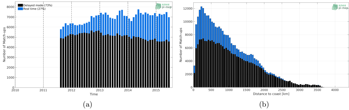
Figure 1: Number of match-ups between Argo and Aquarius-L3-OR-V5-MONTHLY-1DEG SSS as a function of time (a) and as function of the distance to coast (b) over the Mid-Low Latitudes 45N-45S Pi-MEP region and for the full satellite product period.
