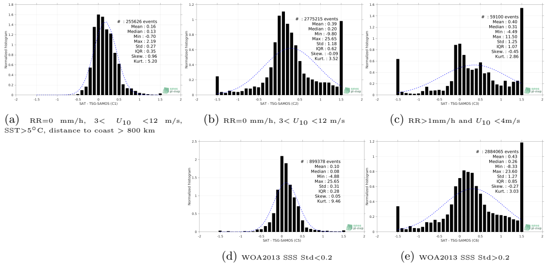
Figure 13: Normalized histogram of \Delta SSS (Aquarius-L3-OR-V5-MONTHLY-RAIN-MASK-1DEG - TSG-SAMOS) for 5 different subdatasets corresponding to: RR=0 mm/h, 3 < U_{10} < 12 m/s, SST >5^\circ\text{C} , distance to coast > 800 km (a), RR=0 mm/h, 3 < U_{10} < 12 m/s (b), RR >1 mm/h and U_{10} < 4 m/s (c), WOA2013 SSS Std <0.2 (d), WOA2013 SSS Std >0.2 (e).
