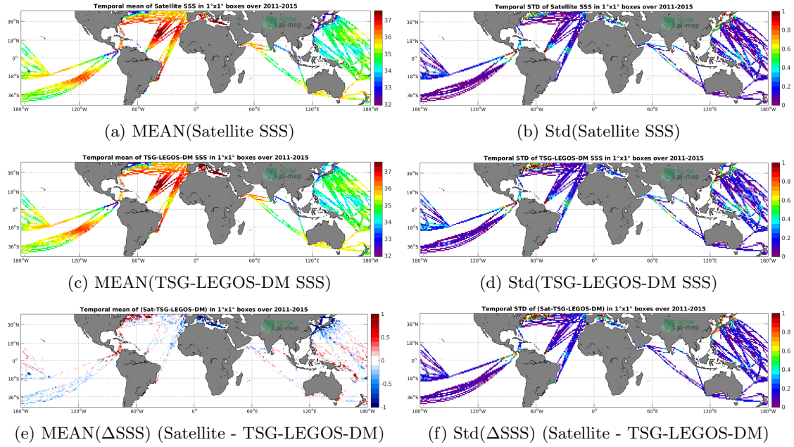
Figure 6: Temporal mean (left) and Std (right) of SSS from Aquarius-L3-OR-V5-MONTHLY-RAIN-MASK-1DEG (top), TSG-LEGOS-DM (middle), and of \Delta SSS (Satellite - TSG-LEGOS-DM). Only match-up pairs are used to generate these maps.
