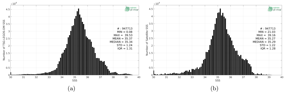
Figure 2: Histograms of SSS from TSG-LEGOS-DM (a) and Aquarius-L3-OR-V5-MONTHLY-RAIN-MASK-1DEG (b) considering all match-up pairs per bins of 0.1 over the Mid-Low Latitudes 45N-45S Pi-MEP region and for the full satellite product period.
