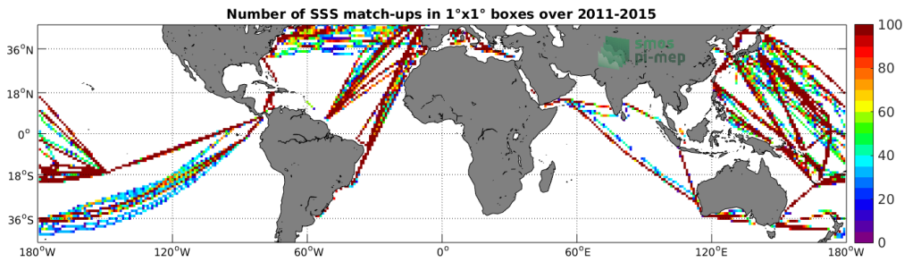
Figure 4: Number of SSS match-ups between TSG-LEGOS-DM SSS and the Aquarius-L3-OR-V5-MONTHLY-RAIN-MASK-1DEG SSS product for the Mid-Low Latitudes 45N-45S Pi-MEP region over 1^\circ \times 1^\circ boxes and for the full satellite product period.
