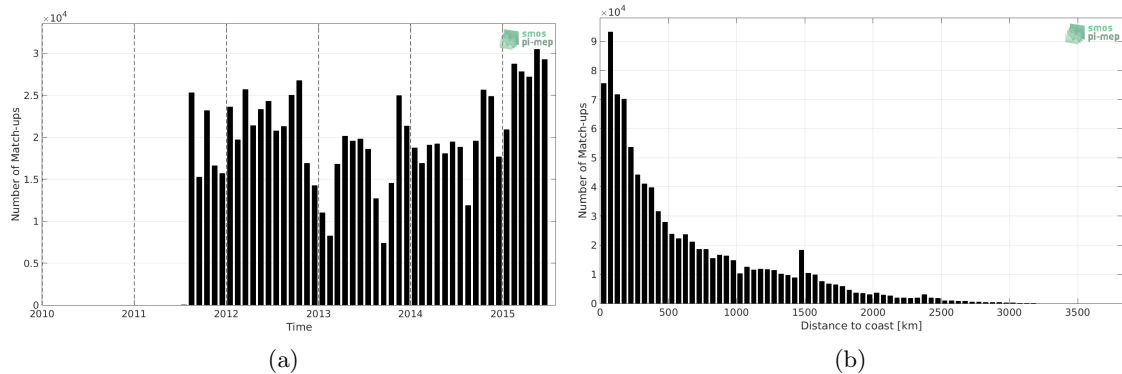
Figure 1: Number of match-ups between TSG-LEGOS-DM and Aquarius-L3-OR-V5-MONTHLY-RAIN-MASK-1DEG SSS as a function of time (a) and as function of the distance to coast (b) over the Mid-Low Latitudes 45N-45S Pi-MEP region and for the full satellite product period.
