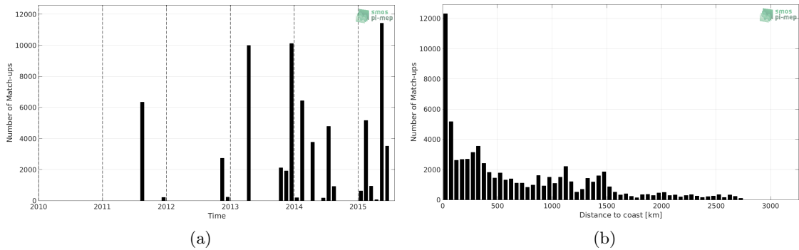
Figure 1: Number of match-ups between TSG-GOSUD-Sailing-ship and Aquarius-L3-OR-V5-MONTHLY-RAIN-MASK-1DEG SSS as a function of time (a) and as function of the distance to coast (b) over the Mid-Low Latitudes 45N-45S Pi-MEP region and for the full satellite product period.
