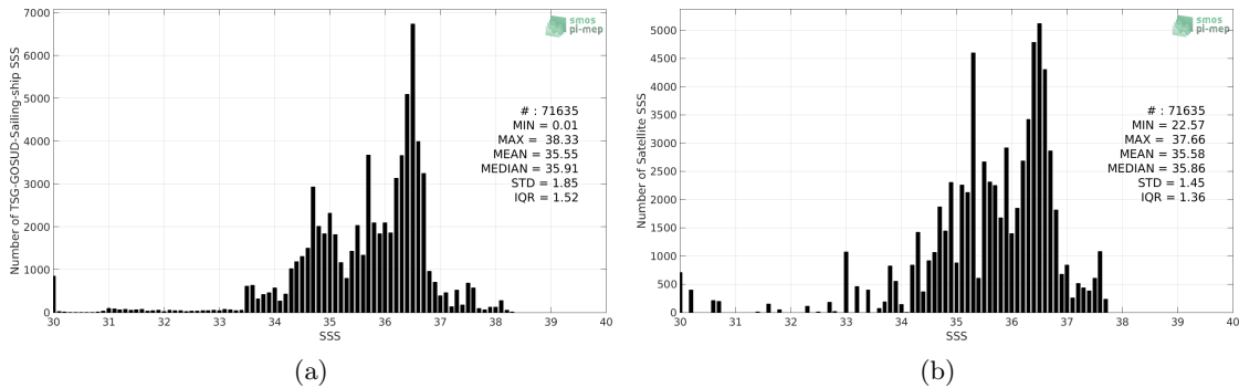
Figure 2: Histograms of SSS from TSG-GOSUD-Sailing-ship (a) and Aquarius-L3-OR-V5-MONTHLY-RAIN-MASK-1DEG (b) considering all match-up pairs per bins of 0.1 over the Mid-Low Latitudes 45N-45S Pi-MEP region and for the full satellite product period.
