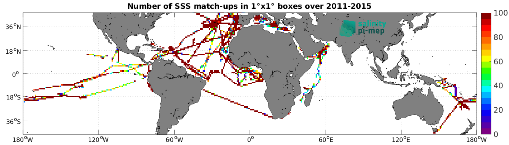
Figure 4: Number of SSS match-ups between TSG (GOSUD-Research-vessel) SSS and the Aquarius SSS L3 OR v5 - Monthly - Rain mask (NASA-GSFC) SSS product for the Mid-Latitudes 45N-45S Pi-MEP region over 1^\circ \times 1^\circ boxes and for the full satellite product period.
