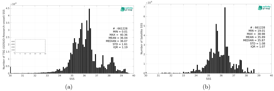
Figure 2: Histograms of SSS from TSG (GOSUD-Research-vessel) (a) and Aquarius SSS L3 OR v5 - Monthly - Rain mask (NASA-GSFC) (b) considering all match-up pairs per bins of 0.1 over the Mid-Low Latitudes 45N-45S Pi-MEP region and for the full satellite product period.
