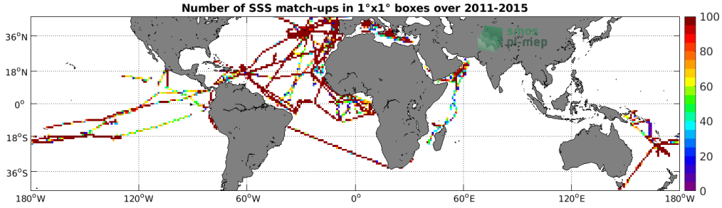
Figure 4: Number of SSS match-ups between TSG (GOSUD-Research-vessel) SSS and the Aquarius SSS L3 OR v5 - Monthly - Rain mask (NASA-GSFC) SSS product for the Mid-Low Latitudes 45N-45S Pi-MEP region over 1^\circ \times 1^\circ boxes and for the full satellite product period.
