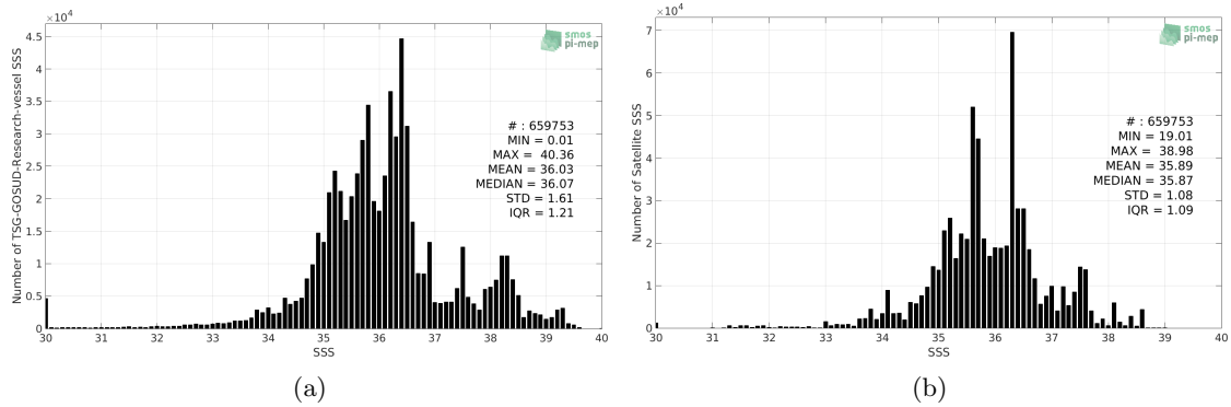
Figure 2: Histograms of SSS from TSG-GOSUD-Research-vessel (a) and Aquarius-L3-OR-V5-MONTHLY-RAIN-MASK-1DEG (b) considering all match-up pairs per bins of 0.1 over the Mid-Low Latitudes 45N-45S Pi-MEP region and for the full satellite product period.
