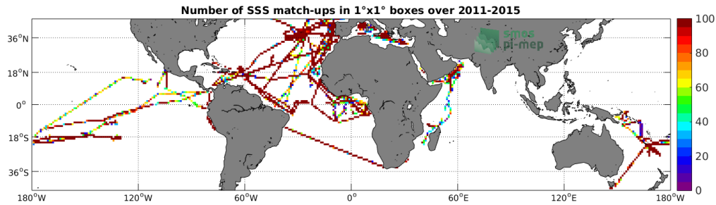
Figure 4: Number of SSS match-ups between TSG-GOSUD-Research-vessel SSS and the Aquarius-L3-OR-V5-MONTHLY-RAIN-MASK-1DEG SSS product for the Mid-Low Latitudes 45N-45S Pi-MEP region over 1°x1° boxes and for the full satellite product period.
