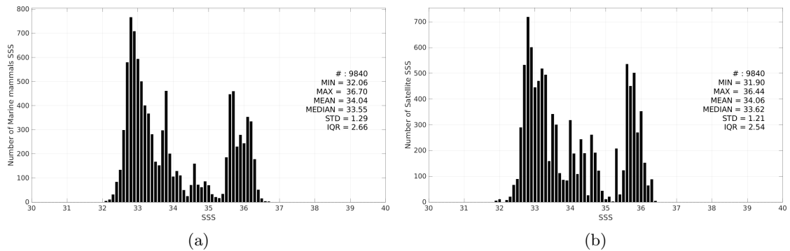
Figure 3: Histograms of SSS from Marine mammals (a) and Aquarius SSS L3 OR v5 - Monthly - Rain mask (NASA-GSFC) (b) considering all match-up pairs per bins of 0.1 over the Mid-Low Latitudes 45N-45S Pi-MEP region and for the full satellite product period.
