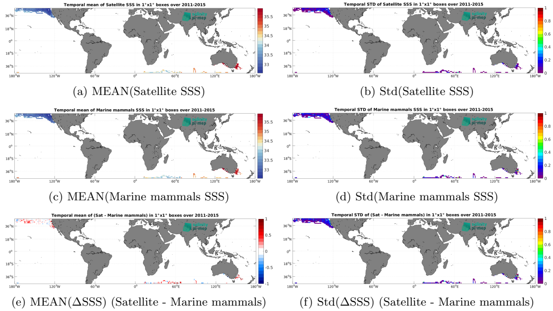
Figure 7: Temporal mean (left) and Std (right) of SSS from Aquarius SSS L3 OR v5 - Monthly - Rain mask (NASA-GSFC) (top), Marine mammals (middle), and of \Delta SSS (Satellite - Marine mammals). Only match-up pairs are used to generate these maps.
