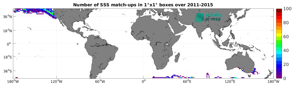
Figure 5: Number of SSS match-ups between Marine mammals SSS and the Aquarius SSS L3 OR v5 - Monthly - Rain mask (NASA-GSFC) SSS product for the Mid-Low Latitudes 45N-45S Pi-MEP region over 1^\circ \times 1^\circ boxes and for the full satellite product period.
