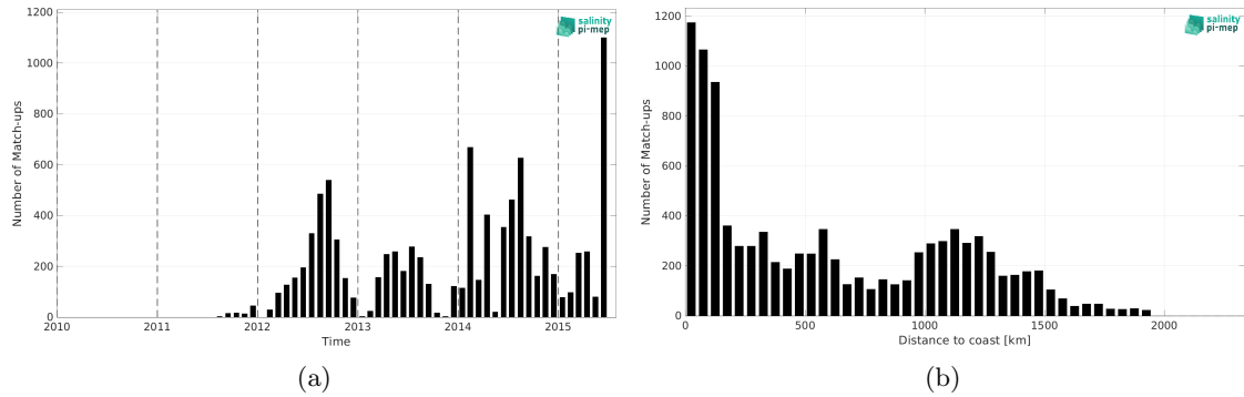
Figure 2: Number of match-ups between Marine mammals and Aquarius SSS L3 OR v5 - Monthly - Rain mask (NASA-GSFC) SSS as a function of time (a) and as function of the distance to coast (b) over the Mid-Low Latitudes 45N-45S Pi-MEP region and for the full satellite product period.
