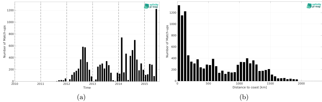
Figure 1: Number of match-ups between Marine mammals and Aquarius SSS L3 OR v5 - Monthly - Rain mask (NASA-GSFC) SSS as a function of time (a) and as function of the distance to coast (b) over the Mid-Low Latitudes 45N-45S Pi-MEP region and for the full satellite product period.
