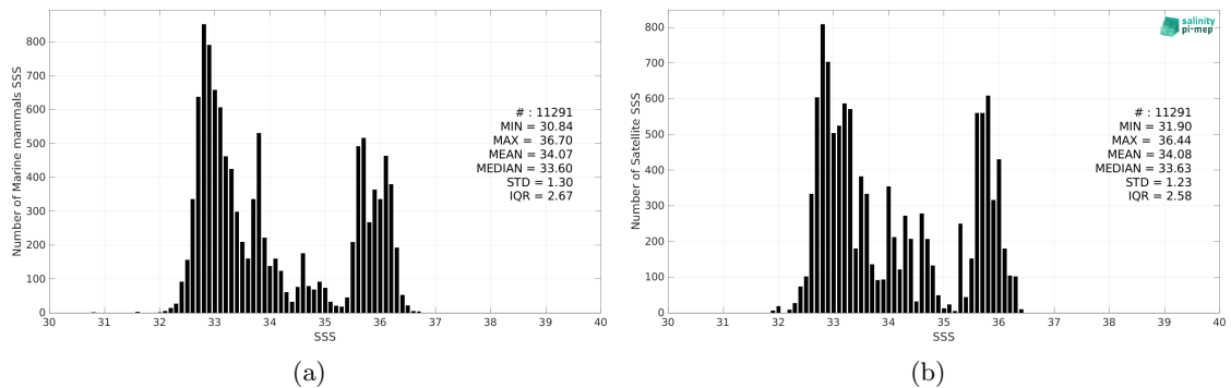
Figure 2: Histograms of SSS from Marine mammals (a) and Aquarius SSS L3 OR v5 - Monthly - Rain mask (NASA-GSFC) (b) considering all match-up pairs per bins of 0.1 over the Mid-Low Latitudes 45N-45S Pi-MEP region and for the full satellite product period.
