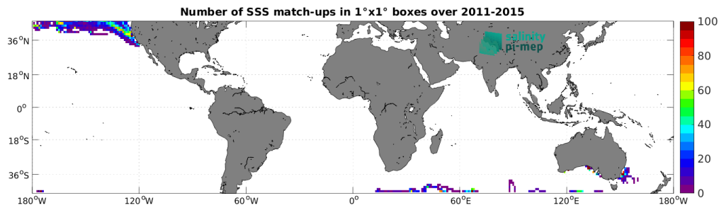
Figure 4: Number of SSS match-ups between Marine mammals SSS and the Aquarius SSS L3 OR v5 - Monthly - Rain mask (NASA-GSFC) SSS product for the Mid-Low Latitudes 45N-45S Pi-MEP region over 1^\circ \times 1^\circ boxes and for the full satellite product period.
