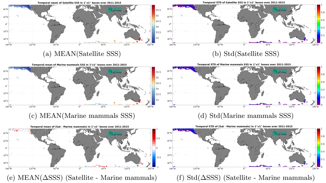
Figure 6: Temporal mean (left) and Std (right) of SSS from Aquarius SSS L3 OR v5 - Monthly - Rain mask (NASA-GSFC) (top), Marine mammals (middle), and of \Delta SSS (Satellite - Marine mammals). Only match-up pairs are used to generate these maps.
