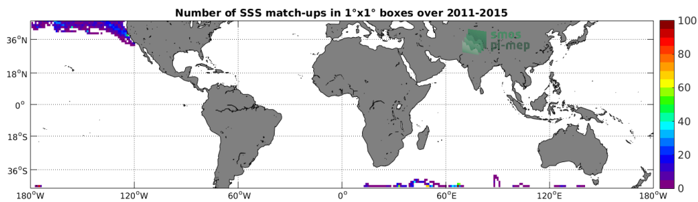
Figure 4: Number of SSS match-ups between Sea mammals SSS and the Aquarius-L3-OR-V5-MONTHLY-RAIN-MASK-1DEG SSS product for the Mid-Low Latitudes 45N-45S Pi-MEP region over 1^\circ \times 1^\circ boxes and for the full satellite product period.
