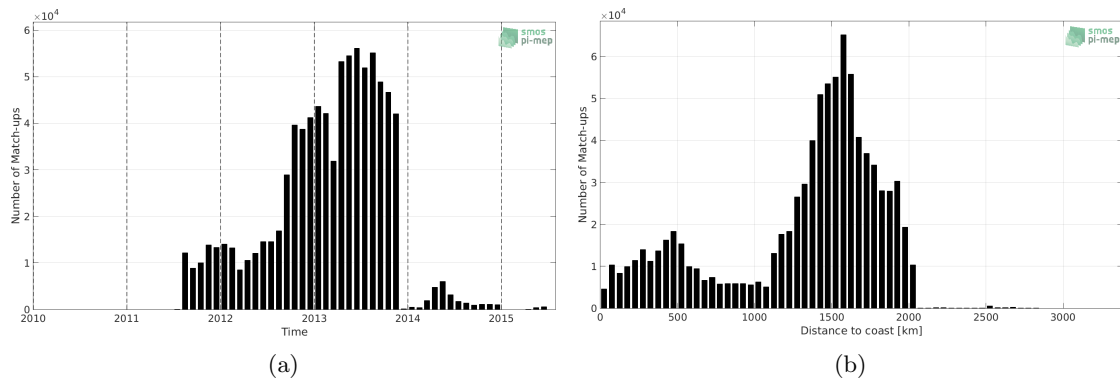
Figure 1: Number of match-ups between Surface drifters and Aquarius-L3-OR-V5-MONTHLY-RAIN-MASK-1DEG SSS as a function of time (a) and as function of the distance to coast (b) over the Mid-Low Latitudes 45N-45S Pi-MEP region and for the full satellite product period.
