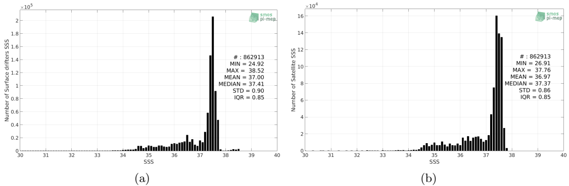
Figure 2: Histograms of SSS from Surface drifters (a) and Aquarius-L3-OR-V5-MONTHLY-RAIN-MASK-1DEG (b) considering all match-up pairs per bins of 0.1 over the Mid-Low Latitudes 45N-45S Pi-MEP region and for the full satellite product period.
