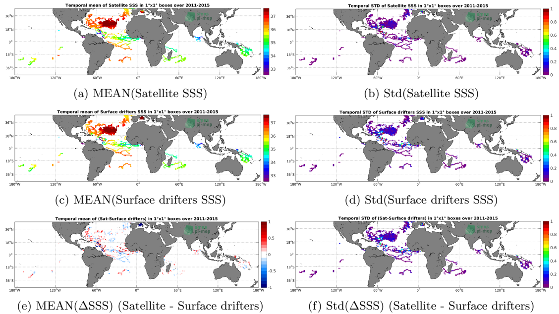
Figure 5: Temporal mean (left) and Std (right) of SSS from Aquarius-L3-OR-V5-MONTHLY-RAIN-MASK-1DEG (top), Surface drifters (middle), and of \Delta SSS (Satellite - Surface drifters). Only match-up pairs are used to generate these maps.
