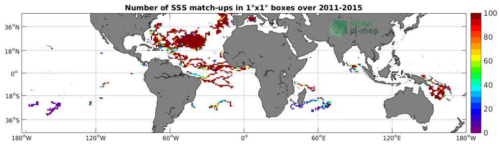
Figure 3: Number of SSS match-ups between Surface drifters SSS and the Aquarius-L3-OR-V5-MONTHLY-RAIN-MASK-1DEG SSS product for the Mid-Low Latitudes 45N-45S Pi-MEP region over 1°x1° boxes and for the full satellite product period.
