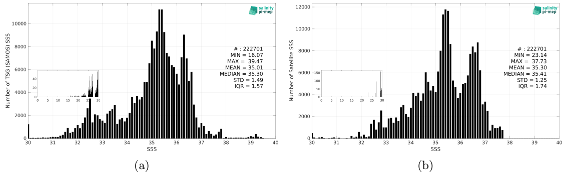
Figure 3: Histograms of SSS from TSG (SAMOS) (a) and Aquarius SSS L3 CAP v5 - 7-Day running (JPL) (b) considering all match-up pairs per bins of 0.1 over the Mid-Low Latitudes 45N-45S Pi-MEP region and for the full satellite product period.
