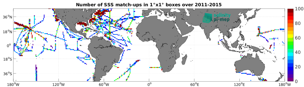
Figure 5: Number of SSS match-ups between TSG (SAMOS) SSS and the Aquarius SSS L3 CAP v5 - 7-Day running (JPL) SSS product for the Mid-Low Latitudes 45N-45S Pi-MEP region over 1^\circ \times 1^\circ boxes and for the full satellite product period.
