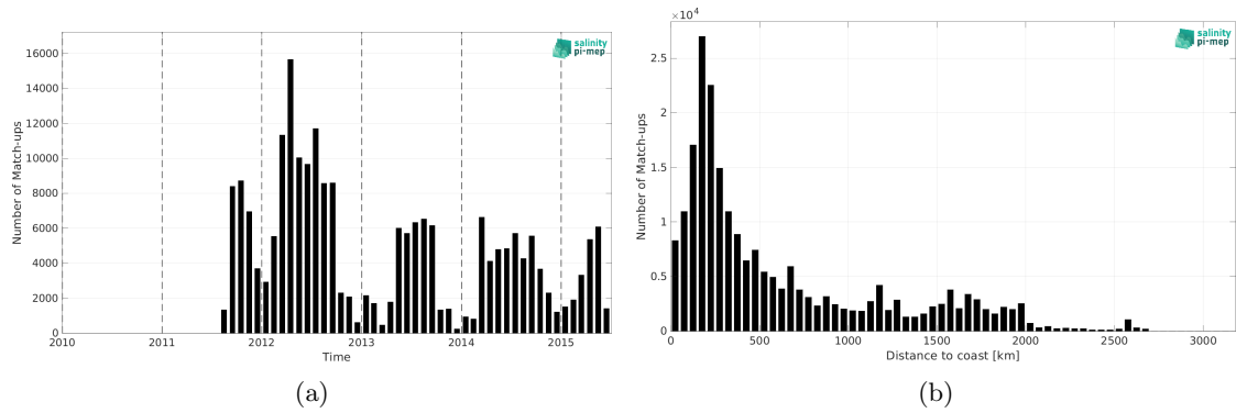
Figure 2: Number of match-ups between TSG (SAMOS) and Aquarius SSS L3 CAP v5 - 7-Day running (JPL) SSS as a function of time (a) and as function of the distance to coast (b) over the Mid-Low Latitudes 45N-45S Pi-MEP region and for the full satellite product period.
