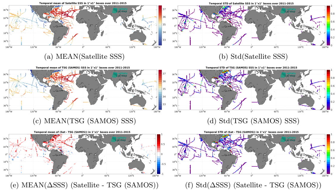
Figure 7: Temporal mean (left) and Std (right) of SSS from Aquarius SSS L3 CAP v5 - 7-Day running (JPL) (top), TSG (SAMOS) (middle), and of \Delta SSS (Satellite - TSG (SAMOS)). Only match-up pairs are used to generate these maps.
