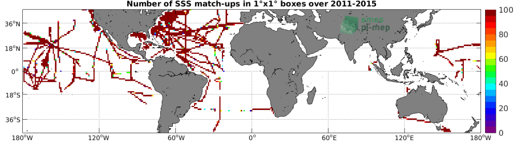
Figure 4: Number of SSS match-ups between TSG (SAMOS) SSS and the Aquarius SSS L3 CAP v5 - 7-Day running (JPL) SSS product for the Mid-Low Latitudes 45N-45S Pi-MEP region over 1°x1° boxes and for the full satellite product period.
