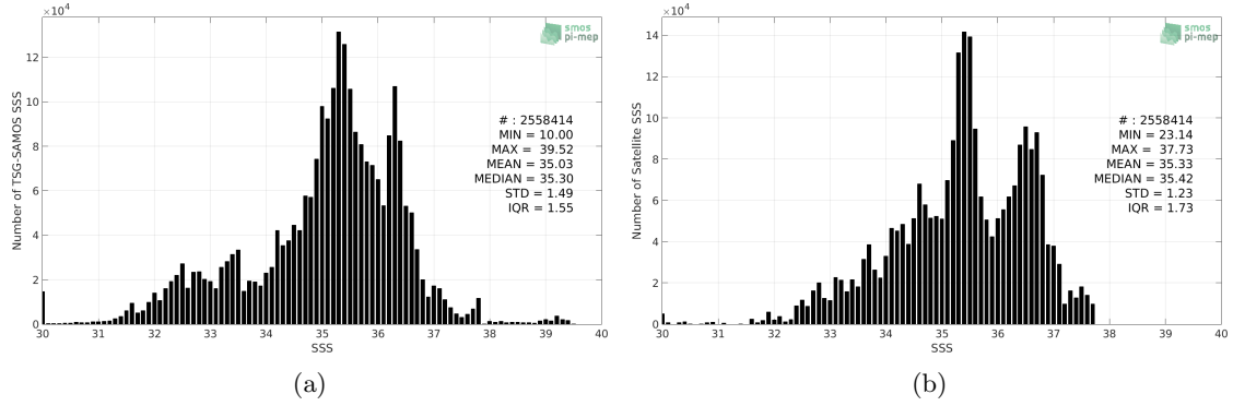
Figure 2: Histograms of SSS from TSG-SAMOS (a) and Aquarius-L3-JPL-V5-7DAY-RUNNING (b) considering all match-up pairs per bins of 0.1 over the Mid-Low Latitudes 45N-45S Pi-MEP region and for the full satellite product period.
