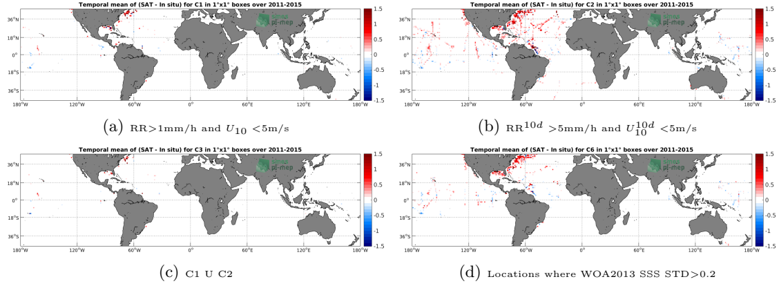
Figure 12: Temporal mean gridded over spatial boxes of size 1^\circ \times 1^\circ of \Delta SSS (Aquarius-L3-JPL-V5-7DAY-RUNNING - TSG-SAMOS) for 4 different subdatasets corresponding to: RR > 1\text{mm/h} and U_{10} < 5\text{m/s} (a), RR^{10d} > 5\text{mm/h} and U_{10}^{10d} < 5\text{m/s} (b), C1 U C2 (c), Locations where WOA2013 SSS STD > 0.2 (d).
