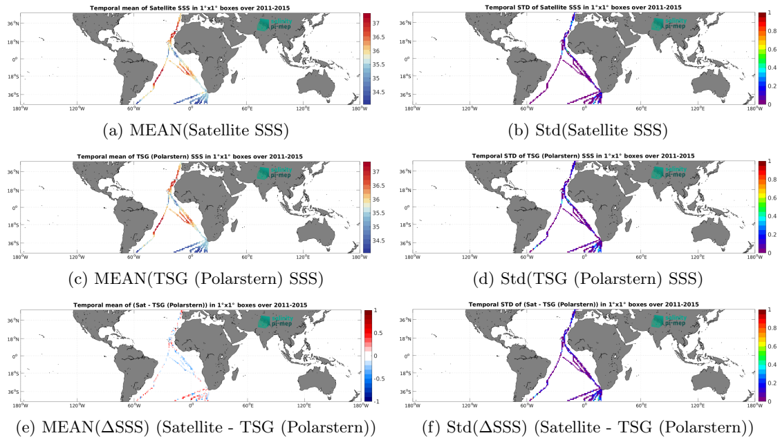
Figure 6: Temporal mean (left) and Std (right) of SSS from Aquarius SSS L3 CAP v5 - 7-Day running (JPL) (top), TSG (Polarstern) (middle), and of \Delta SSS (Satellite - TSG (Polarstern)). Only match-up pairs are used to generate these maps.
