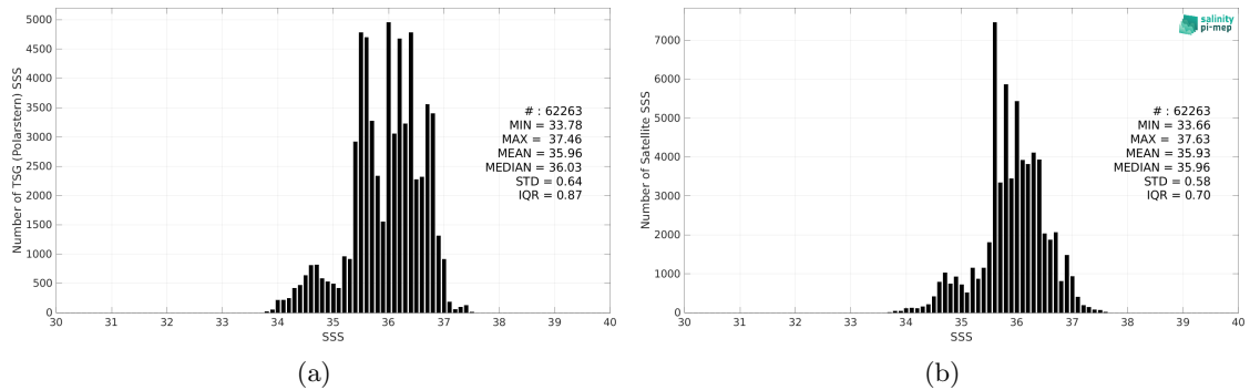
Figure 2: Histograms of SSS from TSG (Polarstern) (a) and Aquarius SSS L3 CAP v5 - 7-Day running (JPL) (b) considering all match-up pairs per bins of 0.1 over the Mid-Low Latitudes 45N-45S Pi-MEP region and for the full satellite product period.
