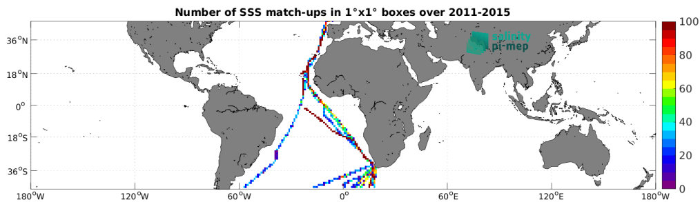
Figure 4: Number of SSS match-ups between TSG (Polarstern) SSS and the Aquarius SSS L3 CAP v5 - 7-Day running (JPL) SSS product for the Mid-Low Latitudes 45N-45S Pi-MEP region over 1^\circ \times 1^\circ boxes and for the full satellite product period.
