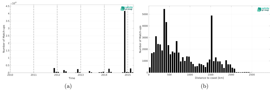
Figure 1: Number of match-ups between TSG (Polarstern) and Aquarius SSS L3 CAP v5 - 7-Day running (JPL) SSS as a function of time (a) and as function of the distance to coast (b) over the Mid-Low Latitudes 45N-45S Pi-MEP region and for the full satellite product period.
