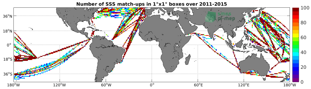
Figure 4: Number of SSS match-ups between TSG (LEGOS-DM) SSS and the Aquarius SSS L3 CAP v5 - 7-Day running (JPL) SSS product for the Mid-Low Latitudes 45N-45S Pi-MEP region over 1°x1° boxes and for the full satellite product period.
