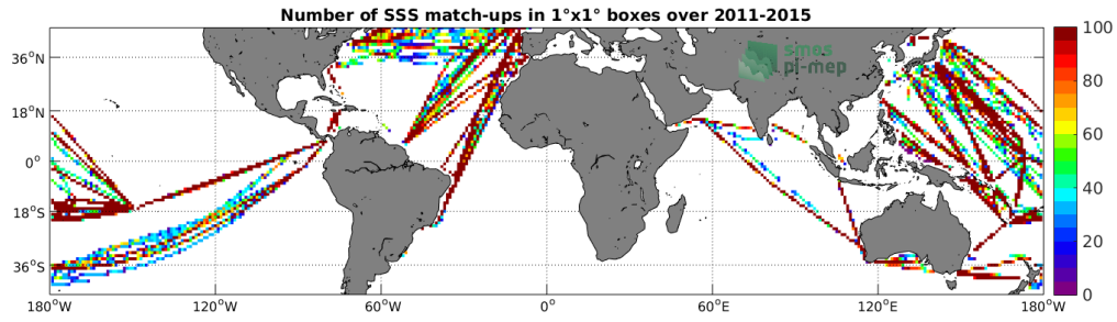
Figure 4: Number of SSS match-ups between TSG-LEGOS-DM SSS and the Aquarius-L3-JPL-V5-7DAY-RUNNING SSS product for the Mid-Low Latitudes 45N-45S Pi-MEP region over 1^\circ \times 1^\circ boxes and for the full satellite product period.
