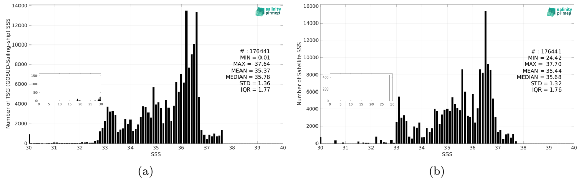
Figure 3: Histograms of SSS from TSG (GOSUD-Sailing-ship) (a) and Aquarius SSS L3 CAP v5 - 7-Day running (JPL) (b) considering all match-up pairs per bins of 0.1 over the Mid-Low Latitudes 45N-45S Pi-MEP region and for the full satellite product period.
