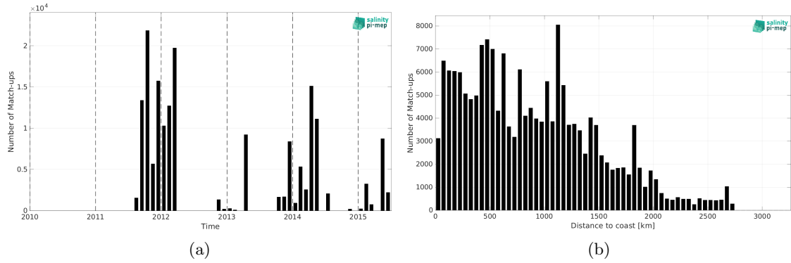
Figure 2: Number of match-ups between TSG (GOSUD-Sailing-ship) and Aquarius SSS L3 CAP v5 - 7-Day running (JPL) SSS as a function of time (a) and as function of the distance to coast (b) over the Mid-Low Latitudes 45N-45S Pi-MEP region and for the full satellite product period.
