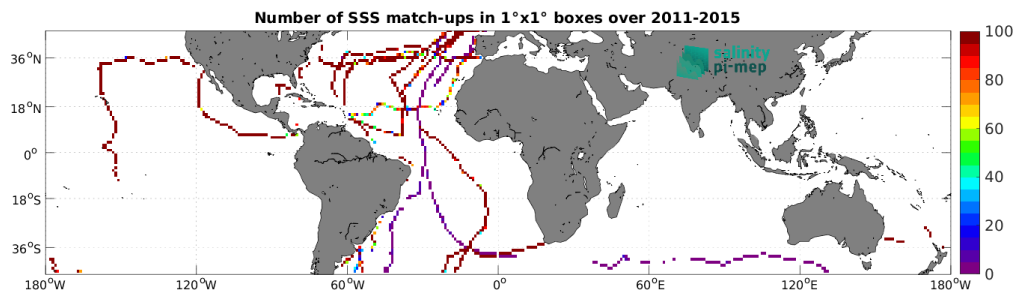
Figure 5: Number of SSS match-ups between TSG (GOSUD-Sailing-ship) SSS and the Aquarius SSS L3 CAP v5 - 7-Day running (JPL) SSS product for the Mid-Low Latitudes 45N-45S Pi-MEP region over 1^\circ \times 1^\circ boxes and for the full satellite product period.
