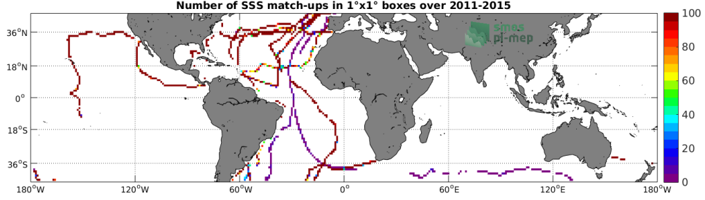
Figure 4: Number of SSS match-ups between TSG-GOSUD-Sailing-ship SSS and the Aquarius-L3-JPL-V5-7DAY-RUNNING SSS product for the Mid-Low Latitudes 45N-45S Pi-MEP region over 1^\circ \times 1^\circ boxes and for the full satellite product period.
