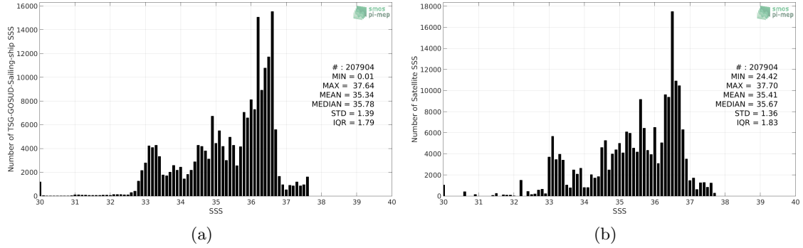
Figure 2: Histograms of SSS from TSG-GOSUD-Sailing-ship (a) and Aquarius-L3-JPL-V5-7DAY-RUNNING (b) considering all match-up pairs per bins of 0.1 over the Mid-Low Latitudes 45N-45S Pi-MEP region and for the full satellite product period.
