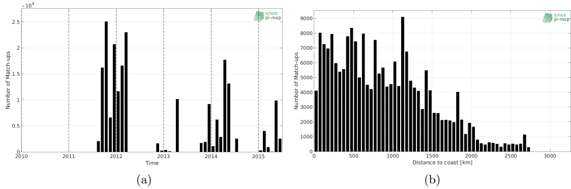
Figure 1: Number of match-ups between TSG-GOSUD-Sailing-ship and Aquarius-L3-JPL-V5-7DAY-RUNNING SSS as a function of time (a) and as function of the distance to coast (b) over the Mid-Low Latitudes 45N-45S Pi-MEP region and for the full satellite product period.
