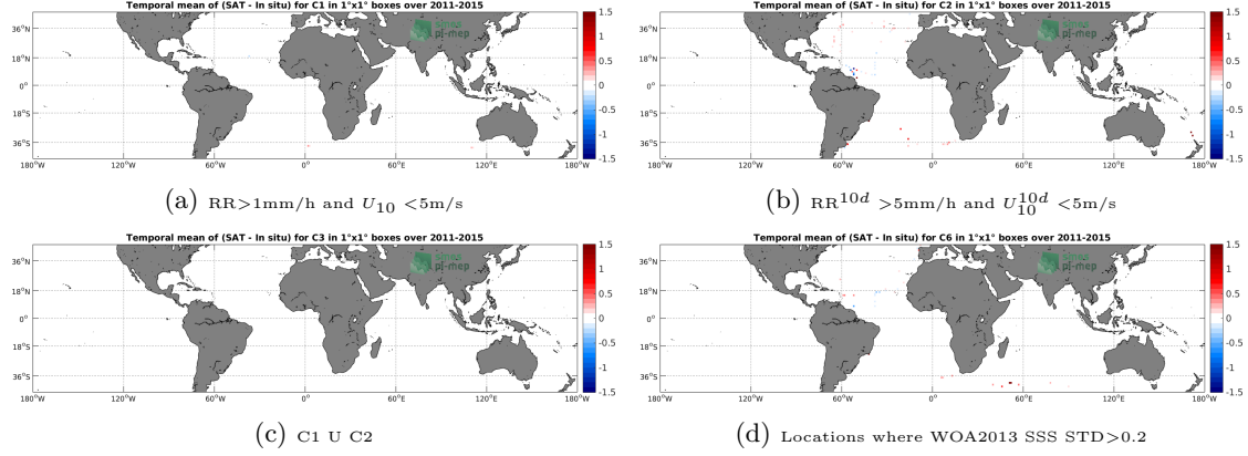
Figure 12: Temporal mean gridded over spatial boxes of size 1^\circ \times 1^\circ of \Delta SSS (Aquarius-L3-JPL-V5-7DAY-RUNNING - TSG-GOSUD-Sailing-ship) for 4 different subdatasets corresponding to: RR > 1\text{mm/h} and U_{10} < 5\text{m/s} (a), RR^{10d} > 5\text{mm/h} and U_{10}^{10d} < 5\text{m/s} (b), C1 U C2 (c), Locations where WOA2013 SSS STD > 0.2 (d).
