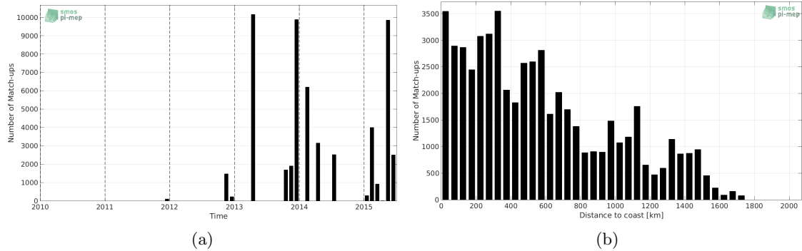
Figure 1: Number of match-ups between TSG-GOSUD-Sailing-ship and Aquarius-L3-JPL-V5-7DAY-RUNNING SSS as a function of time (a) and as function of the distance to coast (b) over the Mid-Low Latitudes 45N-45S Pi-MEP region and for the full satellite product period.
