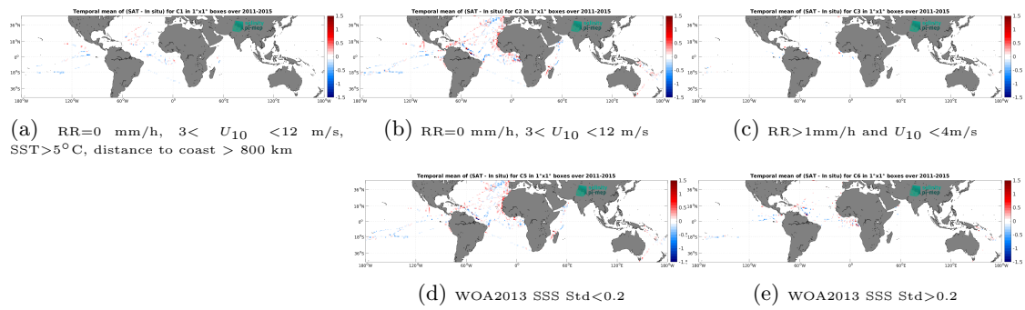
Figure 12: Temporal mean gridded over spatial boxes of size 1^\circ \times 1^\circ of \Delta\text{SSS} (Aquarius SSS L3 CAP v5 - 7-Day running (JPL) - TSG (GOSUD-Research-vessel)) for 5 different subdatasets corresponding to: RR=0 mm/h, 3 < U_{10} < 12 m/s, SST > 5^\circ\text{C} , distance to coast > 800 km (a), RR=0 mm/h, 3 < U_{10} < 12 m/s (b), RR > 1 mm/h and U_{10} < 4 m/s (c), WOA2013 SSS Std < 0.2 (d), WOA2013 SSS Std > 0.2 (e).
