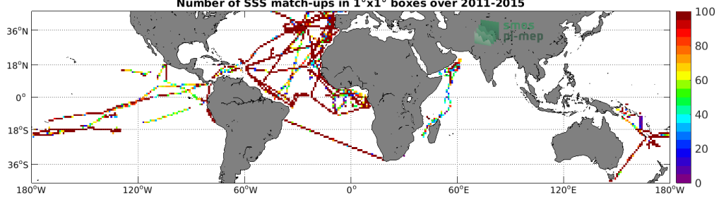
Figure 4: Number of SSS match-ups between TSG (GOSUD-Research-vessel) SSS and the Aquarius SSS L3 CAP v5 - 7-Day running (JPL) SSS product for the Mid-Low Latitudes 45N-45S Pi-MEP region over 1°x1° boxes and for the full satellite product period.
