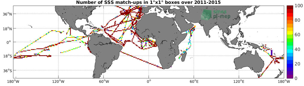
Figure 4: Number of SSS match-ups between TSG-GOSUD-Research-vessel SSS and the Aquarius-L3-JPL-V5-7DAY-RUNNING SSS product for the Mid-Low Latitudes 45N-45S Pi-MEP region over 1°x1° boxes and for the full satellite product period.
