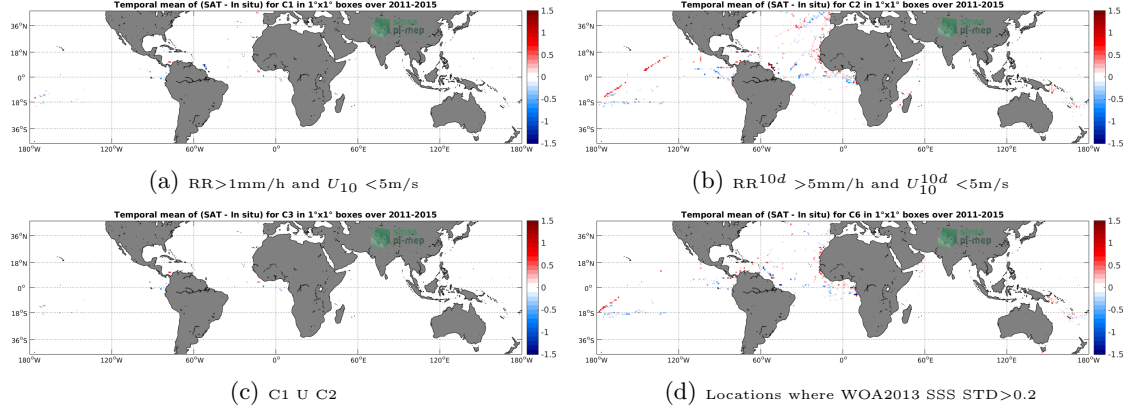
Figure 12: Temporal mean gridded over spatial boxes of size 1^\circ \times 1^\circ of \Delta SSS (Aquarius-L3-JPL-V5-7DAY-RUNNING - TSG-GOSUD-Research-vessel) for 4 different subdatasets corresponding to: RR > 1\text{mm/h} and U_{10} < 5\text{m/s} (a), RR^{10d} > 5\text{mm/h} and U_{10}^{10d} < 5\text{m/s} (b), C1 U C2 (c), Locations where WOA2013 SSS STD > 0.2 (d).
