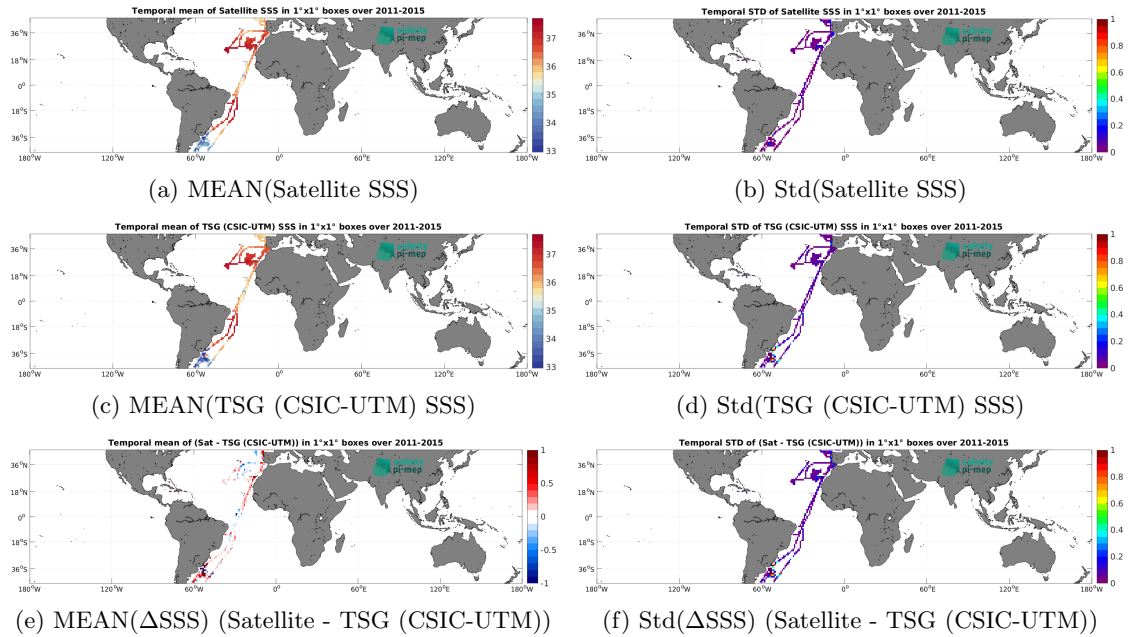
Figure 6: Temporal mean (left) and Std (right) of SSS from Aquarius SSS L3 CAP v5 - 7-Day running (JPL) (top), TSG (CSIC-UTM) (middle), and of \Delta SSS (Satellite - TSG (CSIC-UTM)). Only match-up pairs are used to generate these maps.
