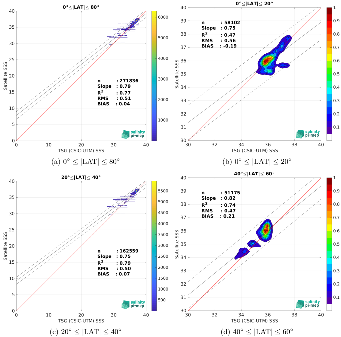
Figure 9: Contour maps of the concentration of Aquarius SSS L3 CAP v5 - 7-Day running (JPL) SSS ( y -axis) versus TSG (CSIC-UTM) SSS ( x -axis) at match-up pairs for different latitude bands. For each plot, the red line shows x=y . The black thin and dashed lines indicate a linear fit through the data cloud and the \pm 95\% confidence levels, respectively. The number match-up pairs n , the slope and R^2 coefficient of the linear fit, the root mean square (RMS) and the mean bias between satellite and in situ data are indicated for each latitude band in each plots.
