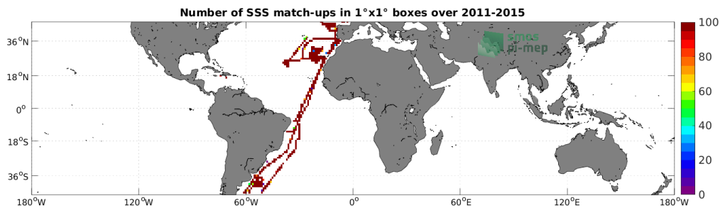
Figure 4: Number of SSS match-ups between TSG (CSIC-UTM) SSS and the Aquarius SSS L3 CAP v5 - 7-Day running (JPL) SSS product for the Mid-Low Latitudes 45N-45S Pi-MEP region over 1^\circ \times 1^\circ boxes and for the full satellite product period.
