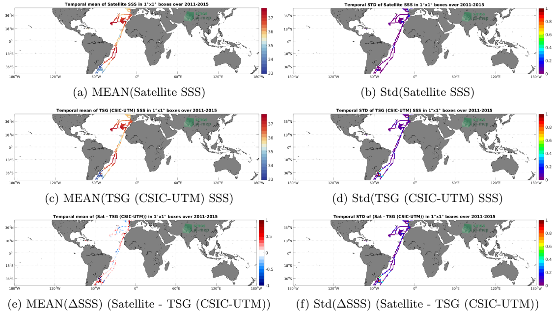
Figure 6: Temporal mean (left) and Std (right) of SSS from Aquarius SSS L3 CAP v5 - 7-Day running (JPL) (top), TSG (CSIC-UTM) ( in situ ) dataset (middle), and of \Delta SSS (Satellite - TSG (CSIC-UTM)). Only match-up pairs are used to generate these maps.
