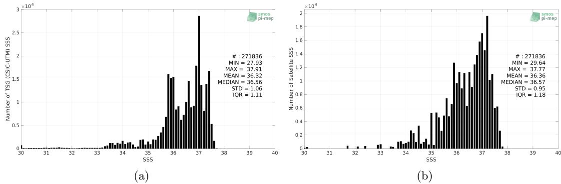
Figure 2: Histograms of SSS from TSG (CSIC-UTM) (a) and Aquarius SSS L3 CAP v5 - 7-Day running (JPL) (b) considering all match-up pairs per bins of 0.1 over the Mid-Low Latitudes 45N-45S Pi-MEP region and for the full satellite product period.
