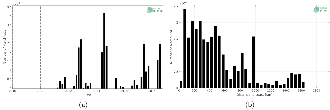
Figure 1: Number of match-ups between TSG (CSIC-UTM) and Aquarius SSS L3 CAP v5 - 7-Day running (JPL) SSS as a function of time (a) and as function of the distance to coast (b) over the Mid-Low Latitudes 45N-45S Pi-MEP region and for the full satellite product period.
