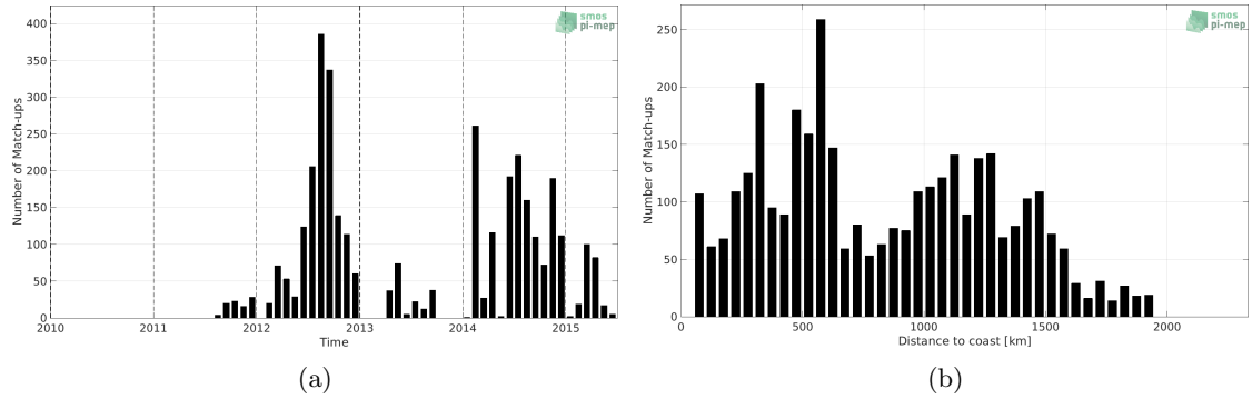
Figure 1: Number of match-ups between Sea mammals and Aquarius SSS L3 CAP v5 - 7-Day running (JPL) SSS as a function of time (a) and as function of the distance to coast (b) over the Mid-Low Latitudes 45N-45S Pi-MEP region and for the full satellite product period.
