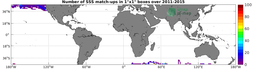
Figure 4: Number of SSS match-ups between Sea mammals SSS and the Aquarius SSS L3 CAP v5 - 7-Day running (JPL) SSS product for the Mid-Low Latitudes 45N-45S Pi-MEP region over 1°x1° boxes and for the full satellite product period.
