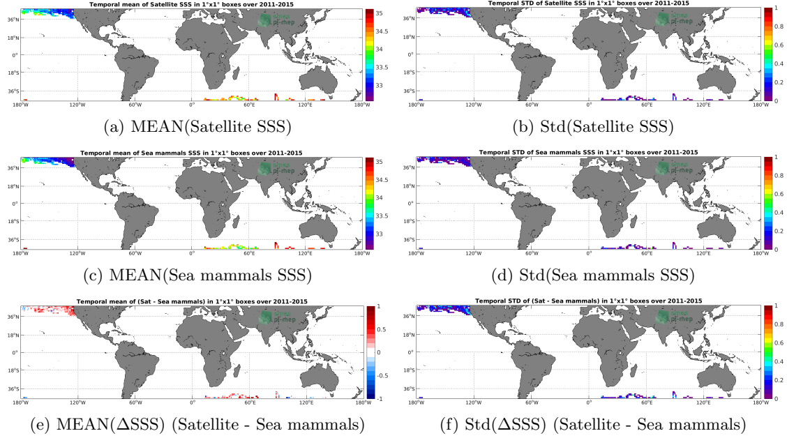
Figure 6: Temporal mean (left) and Std (right) of SSS from Aquarius SSS L3 CAP v5 - 7-Day running (JPL) (top), Sea mammals (middle), and of \Delta SSS (Satellite - Sea mammals). Only match-up pairs are used to generate these maps.
