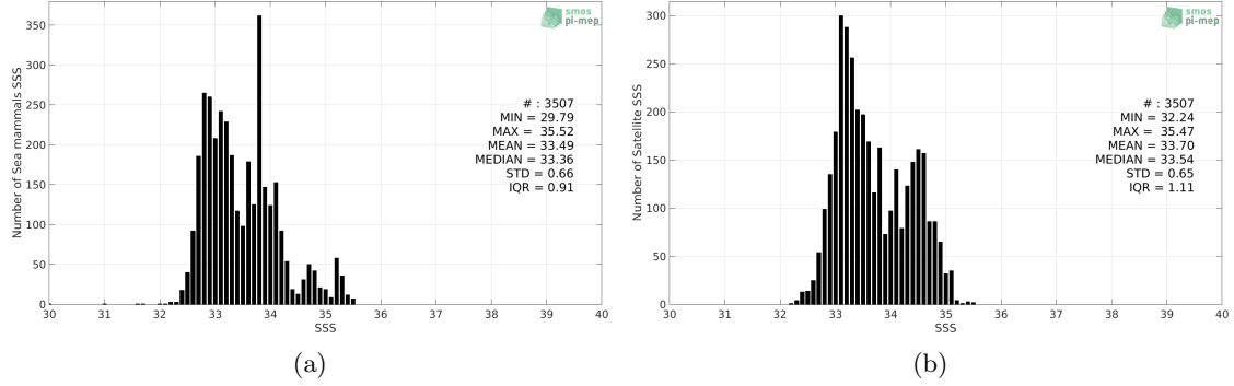
Figure 2: Histograms of SSS from Sea mammals (a) and Aquarius SSS L3 CAP v5 - 7-Day running (JPL) (b) considering all match-up pairs per bins of 0.1 over the Mid-Low Latitudes 45N-45S Pi-MEP region and for the full satellite product period.
