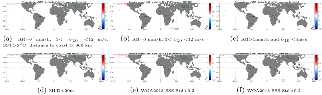
Figure 12: Temporal mean gridded over spatial boxes of size 1^\circ \times 1^\circ of \Delta SSS (Aquarius SSS L3 CAP v5 - 7-Day running (JPL) - Sea mammals) for 6 different subdatasets corresponding to: RR=0 mm/h, 3 < U_{10} < 12 m/s, SST > 5^\circ C , distance to coast > 800 km (a), RR=0 mm/h, 3 < U_{10} < 12 m/s (b), RR > 1 mm/h and U_{10} < 4 m/s (c), MLD < 20 m (d), WOA2013 SSS Std < 0.2 (e), WOA2013 SSS Std > 0.2 (f).
