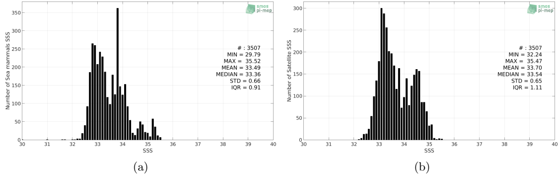
Figure 2: Histograms of SSS from Sea mammals (a) and Aquarius-L3-JPL-V5-7DAY-RUNNING (b) considering all match-up pairs per bins of 0.1 over the Mid-Low Latitudes 45N-45S Pi-MEP region and for the full satellite product period.
