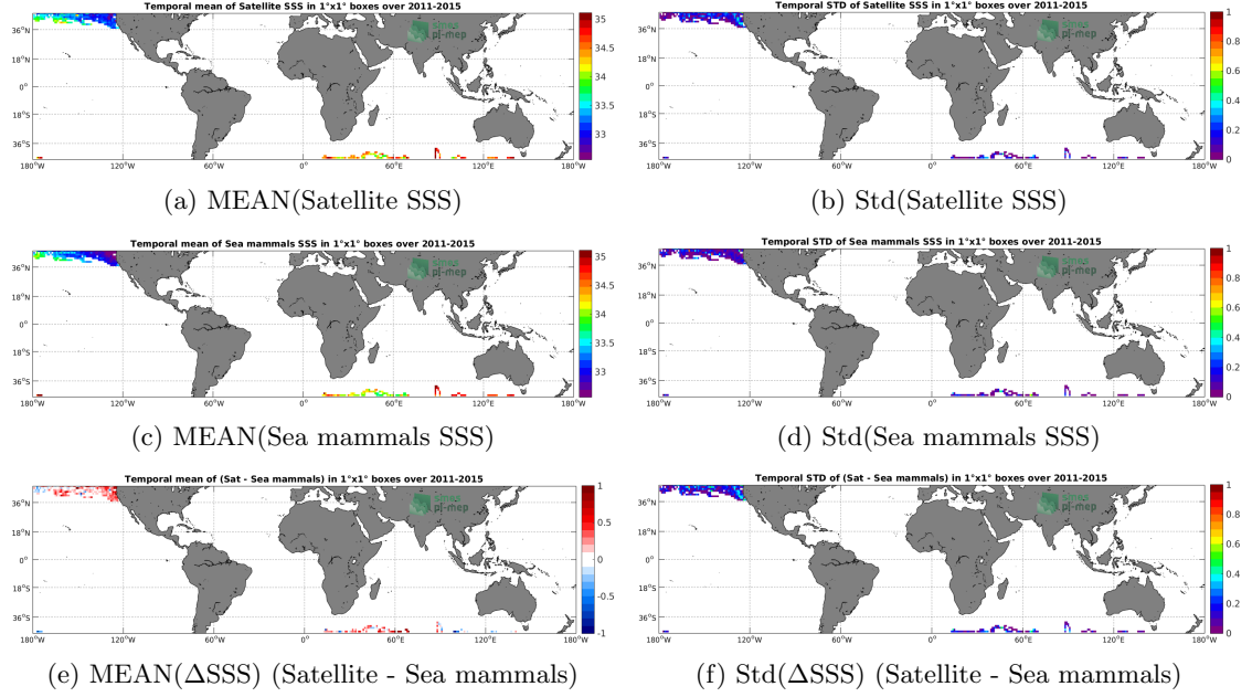
Figure 6: Temporal mean (left) and Std (right) of SSS from Aquarius-L3-JPL-V5-7DAY-RUNNING (top), Sea mammals (middle), and of \Delta SSS (Satellite - Sea mammals). Only match-up pairs are used to generate these maps.
