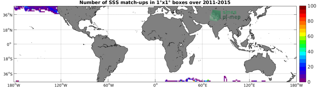
Figure 4: Number of SSS match-ups between Sea mammals SSS and the Aquarius-L3-JPL-V5-7DAY-RUNNING SSS product for the Mid-Low Latitudes 45N-45S Pi-MEP region over 1^\circ \times 1^\circ boxes and for the full satellite product period.
