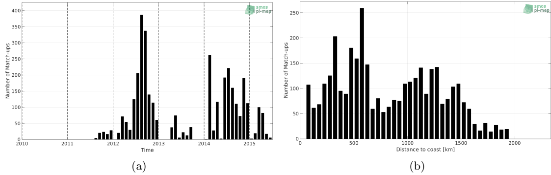
Figure 1: Number of match-ups between Sea mammals and Aquarius-L3-JPL-V5-7DAY-RUNNING SSS as a function of time (a) and as function of the distance to coast (b) over the Mid-Low Latitudes 45N-45S Pi-MEP region and for the full satellite product period.
